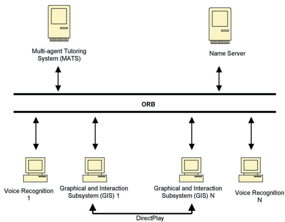
Figure 4 MAEVIF's System Architecture.
