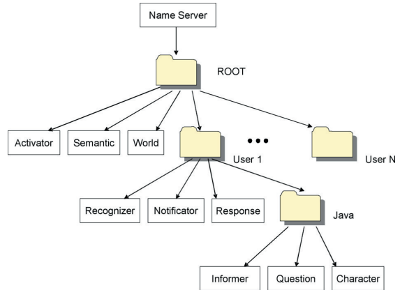
Figure 5 Name contexts structure in MAEVIF.
