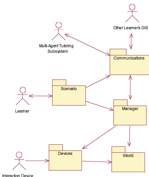
Figure 1 Packages in the graphics and interaction subsystem of MAEVIF.
