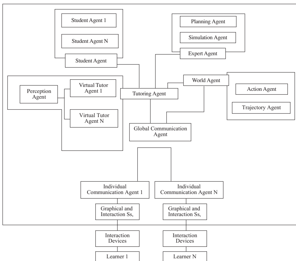
Figure 3 MAEVIF Multi-agent Architecture.
