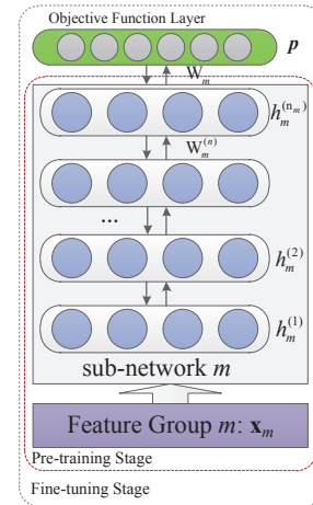
Fig. 3. Illustration of the structure of the sub-networks. In the pre-training stage, we train the branch sub-networks (including those layers in the red box) as stacked denoising auto-encoders layer-wisely. In the fine-tuning stage, we train the branches and the shared objective function layer overall as multilayer perceptron with back-propagation.
