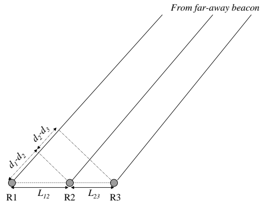
Figure 5: Using three receivers to measure (d_1 - d_2) .
