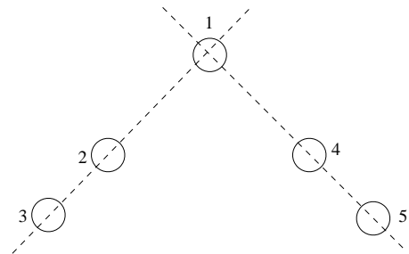
Figure 8: Five receivers on a compass forming two perpendicular receiver-triplets, which are used to unambiguously infer the heading with respect to a beacon.
