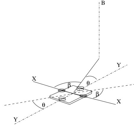
Figure 7: Two sets of receivers can break the symmetry. One set of receiver triplets lies on the X-X line and the second set lies on the Y-Y line.
