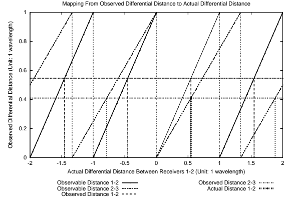
Figure 10: Finding the actual differential distance between R_1 and R_2 by using the observed differential distances from (R_1, R_2) and (R_2, R_3) .
