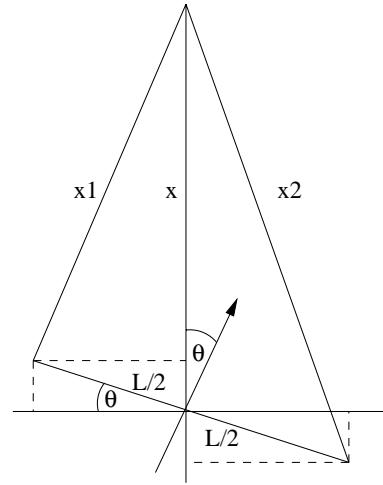
Figure 3: A rotated compass leads to a difference in distances between the beacon and each of the receivers. This figure is the result of projecting the beacon onto the horizontal plane of the compass.
