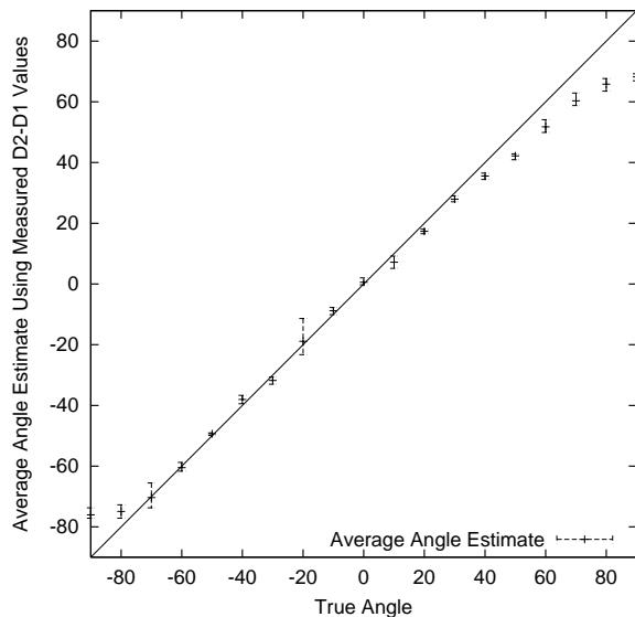
Figure 11: Average angle estimates versus true angle values. The error bars indicate the absolute angle errors for all three trials. The line y = x plots the ideal relationship between the true and estimated angle values.
