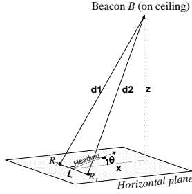
Figure 2: Determining the angle of orientation along the horizontal plane, \theta , using distance estimates. Observe that the heading is perpendicular to the line joining the ultrasonic compass receivers, R_1 and R_2 , which are placed at a distance L from each other.
