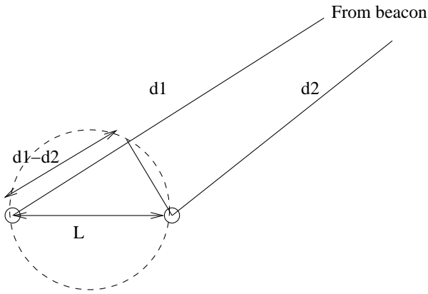
Figure 4: Receivers R_1 and R_2 can measure the differential distance from a far-away beacon.
