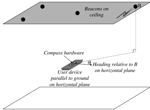
Figure 1: Setup of beacons on the ceiling of a room and a user device with attached compass hardware. The Cricket compass solves the problem of obtaining the precise position and orientation of the user device relative to a coordinate system defined by the beacons.
