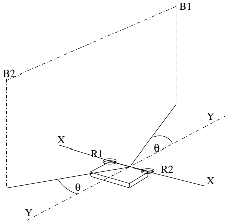
Figure 6: \theta is ambiguous—the beacon can be at either B_1 or B_2 .
