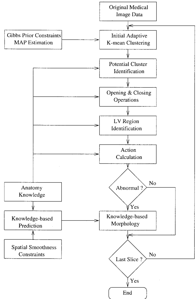
Fig. 3. Block diagram of the overall 3-D segmentation scheme.
