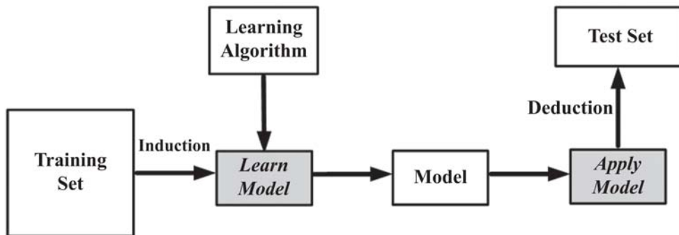
Figure 5.2: Supervised Learning.
