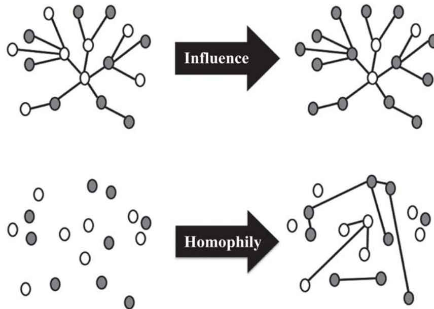
Figure 8.1: Influence and Homophily.
