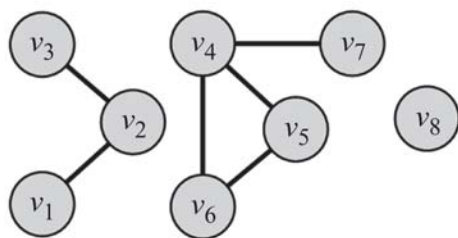
Figure 10.5: Neighborhood-Based Link Prediction Example.
