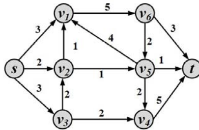
Figure 2.31: Flow Graph
