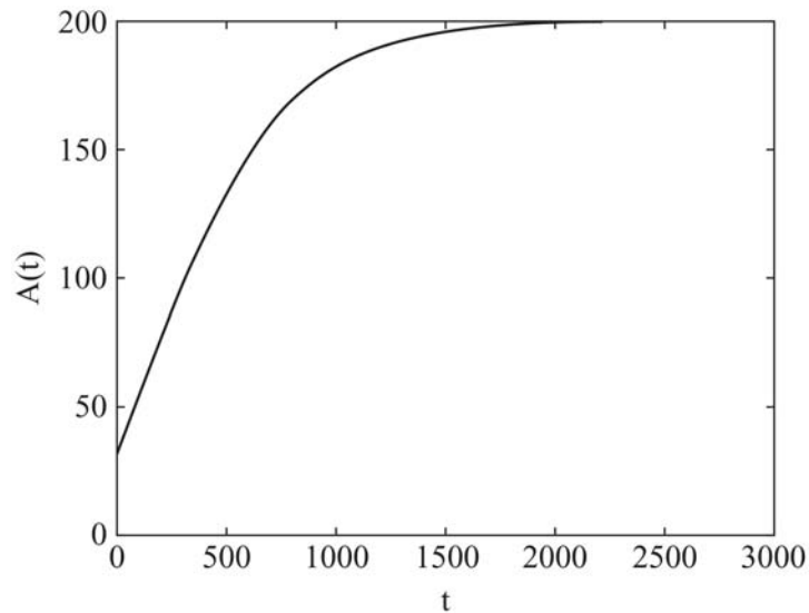
Figure 7.9: Mixed-Influence Model for P = 200 , \beta = 10^{-5} , A_0 = 30 , and \alpha = 10^{-3} .
