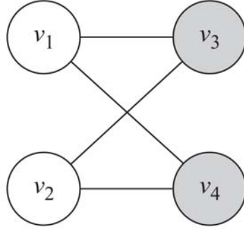
Figure 8.3: A Modularity Example for a Bipartite Graph.
