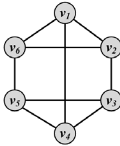
Figure 2.17: Regular Graph with k = 3 .
