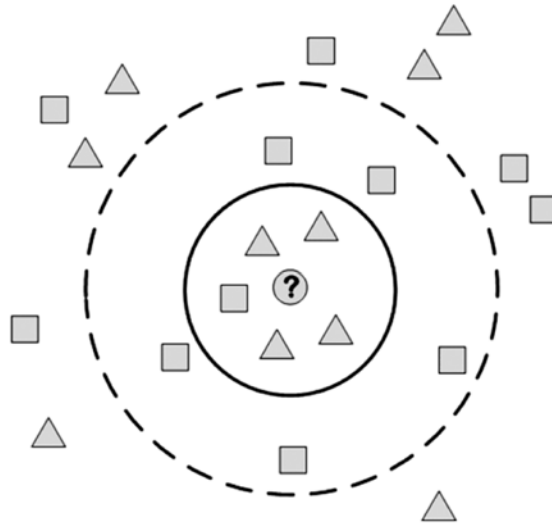
Figure 5.4: k -Nearest Neighbor Example. In this figure, our goal is to predict the label for the instance shown using a circle. When k = 5 , the predicted label is ▲ and when k = 9 the predicted label is ■.
