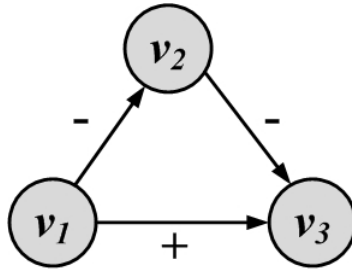
Figure 2.5: A Signed Graph Example.
