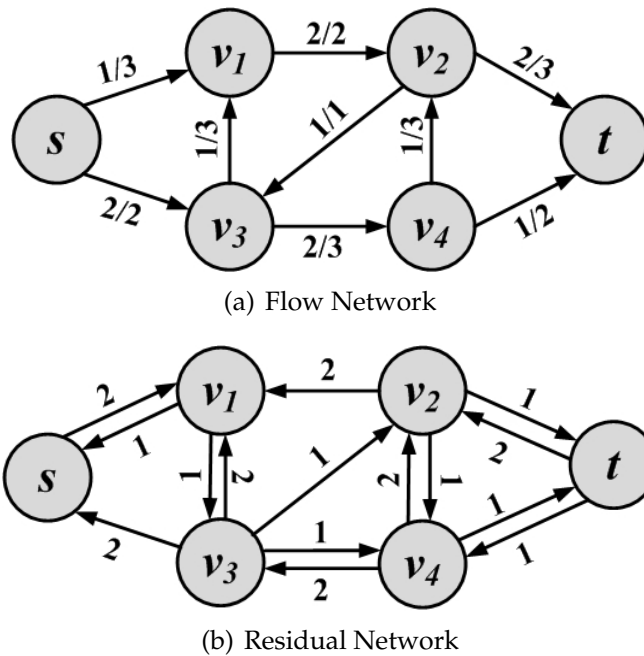
Figure 2.24: A Flow Network and Its Residual.
