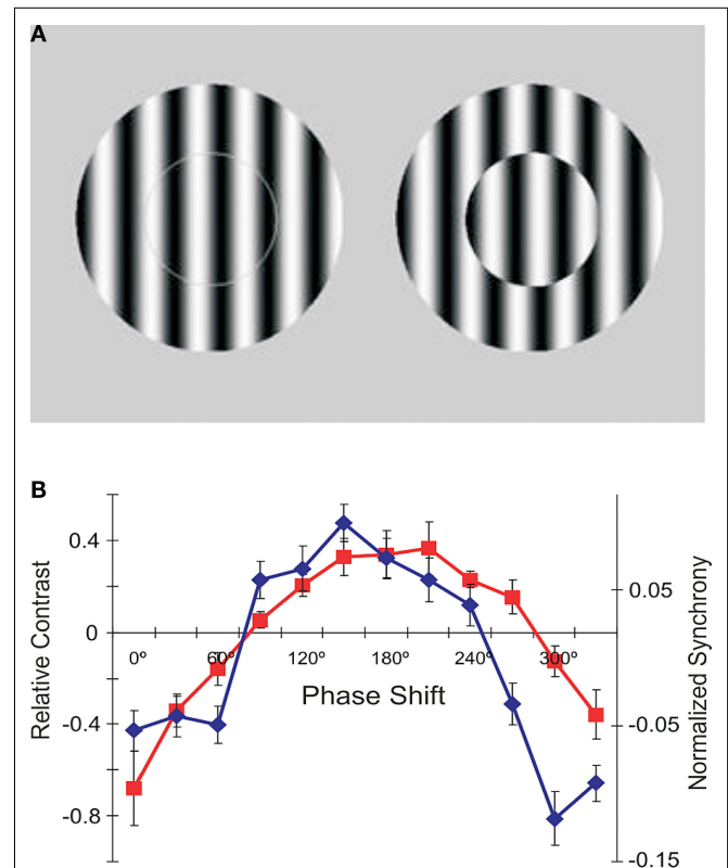
FIGURE 4 | The role of synchrony for perception of brightness. (A) In the two centre-surround stimuli, the gratings in the centre are physical identical. Nevertheless, most observers report seeing stronger contrast on the right where the centre is offset for 180° relative to the surround. (B) Experimental results obtained with stimuli shown in (A) . Red: Human psychophysical judgments of changes in perceived contrast as a function of phase offset between the centre and surround. Blue: Changes in the strength of synchronization between neurons in cat area 17 whose receptive fields were covered by the centre stimuli and whose orientation preferences matched the orientation of the grating. Adapted from Biederlack et al. (2006).
