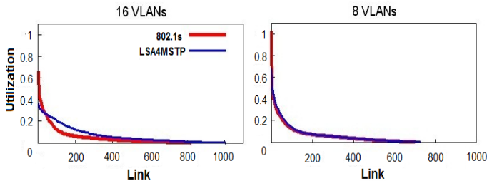
Fig. 4: Link utilization distribution
