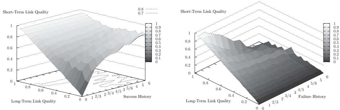
(a) Influence of recent transmission success rate on short-term link quality. A label of k/h stands for k successes during the last h transmissions, and h is a shorthand for h/h .
