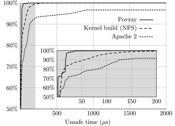
Figure 3. Cumulative probability of unsafe state times for three different workloads. The two graphs show the probabilities of both long and short unsafe state times.
