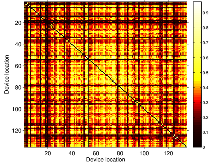
Figure 1: Correlation coefficients of the raw traces from the Building 1 dataset (Section 4.1). The matrix is ordered such as the devices serving same/adjacent rooms are nearby in the matrix.
