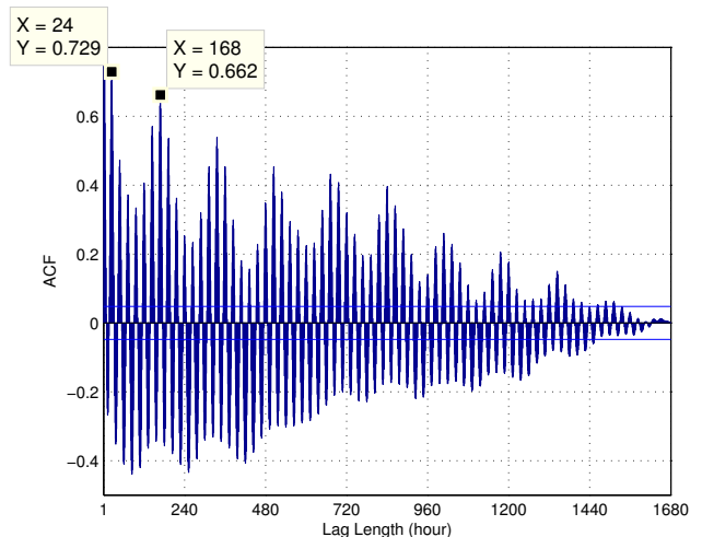
Figure 2: Auto-correlation of a usual signal from the Building 1 dataset. The signal features daily and weekly patterns (resp. x = 24 and x = 168 ).
