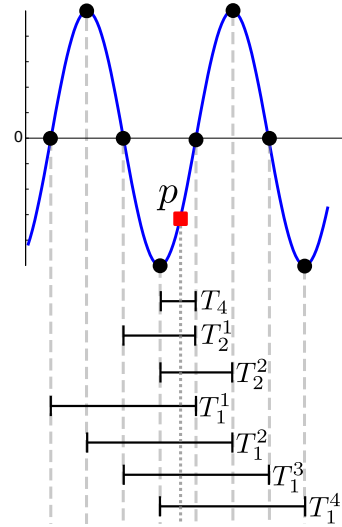
Figure 4: Generalized Zero Crossing: the local mean period at the point p is computed from one quarter period T_4 , two half periods T_2^x and four full periods T_1^y (where x = 1, 2 , and, y = 1, 2, 3, 4 ).
