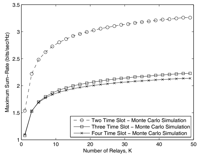
Fig. 10. Maximum sum-rate of the two, three and four time slot opportunistic relay scheme with \bar{\gamma}_A = \bar{\gamma}_r = 10 dB, and \bar{\gamma}_B = 20 dB.
