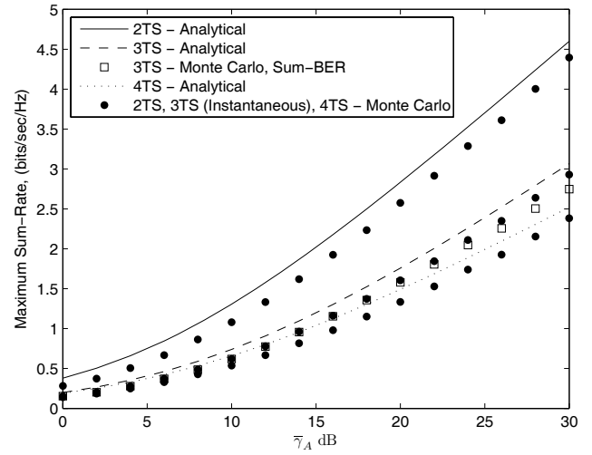
Fig. 4. Maximum sum-rate of the two, three and four time slot schemes with \bar{\gamma}_B = 0.5\bar{\gamma}_A and \bar{\gamma}_r = 0.8\bar{\gamma}_A .
