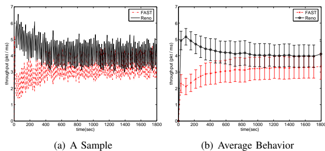
Fig. 11. FAST vs. Reno, with buffer size of 400 pkts.
