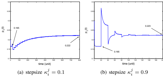
Fig. 8. Case 1: p_1(t) with different \kappa_i^j
