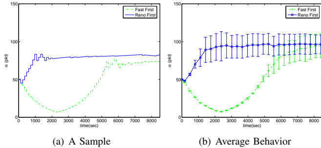
Fig. 16. \alpha trajectory of example 2b
