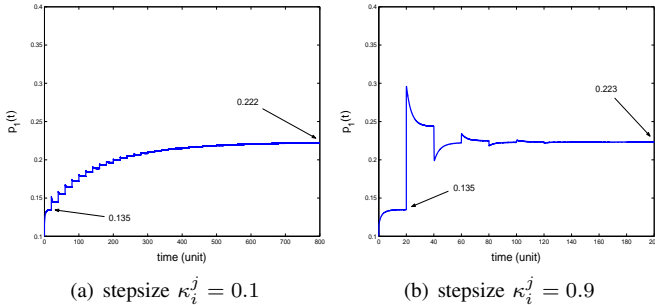
Fig. 9. Case 2: p_1(t) with different \kappa_i^j
