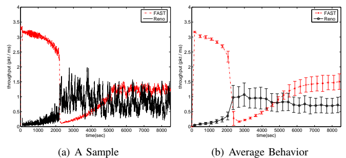
Fig. 14. FAST starts first.
