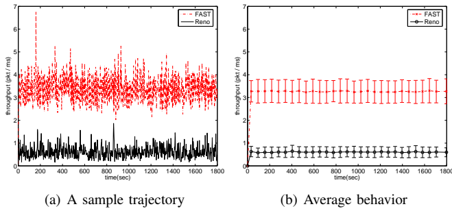
Fig. 3. FAST vs. Reno with a buffer size of 80 pkts.
