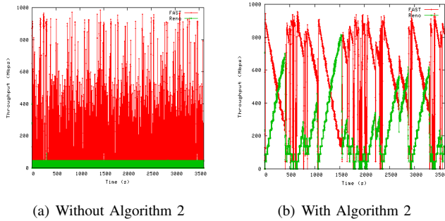
Fig. 19. Bandwidth partition between Reno and FAST
