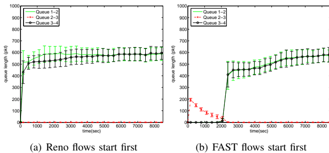
Fig. 17. Trajectories of queues of example 2b
