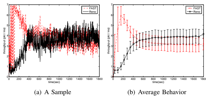
Fig. 12. FAST vs. Reno, with buffer size of 80 pkts.
