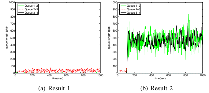
Fig. 18. Trajectories of queues of example 2a, with \alpha fixed at 8.2 and using different random seeds (FAST flows start first)
