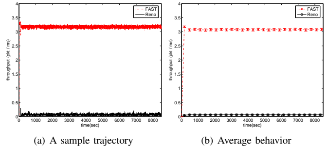
Fig. 5. Bandwidth shares of Reno and FAST when FAST starts first.
