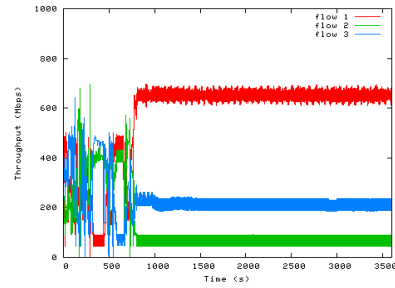
Fig. 20. Bandwidth sharing among FAST flows
