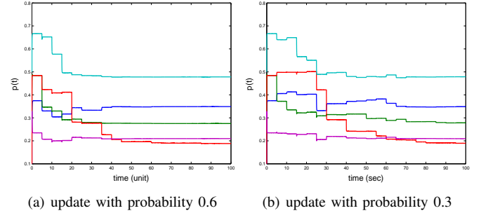
Fig. 10. p(t) with different probability of updating
