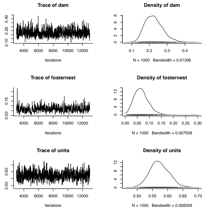
Figure 3.1: MCMC summary plot for the variance components from model m3a.1 .
