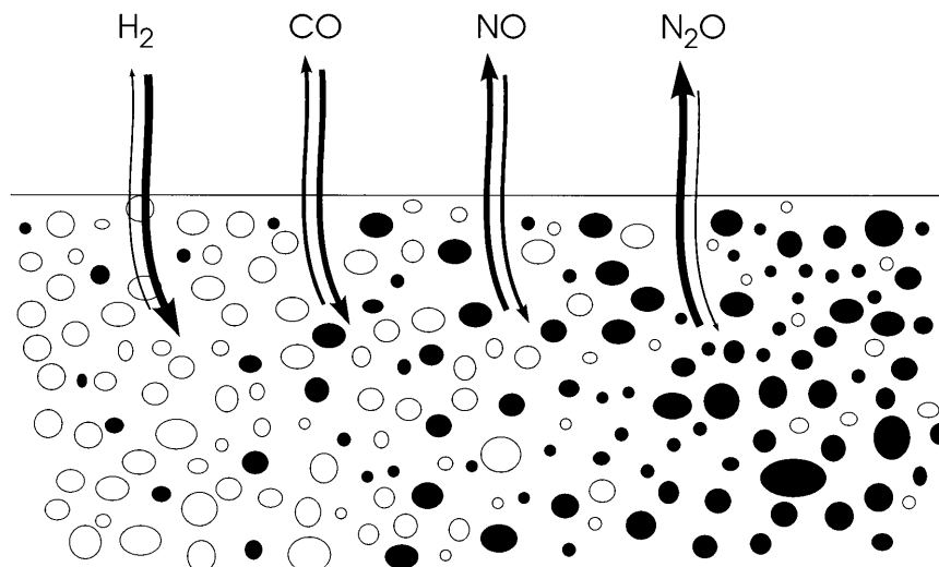
FIG. 5. Conceptual scheme of the bidirectional fluxes of H 2 , CO, NO, and N 2 O between the upland soil and atmosphere as a result of the relative amounts of soil entities (e.g., soil crumbs) that either release trace gas into the soil atmosphere (open symbols) or take it up (solid symbols).
