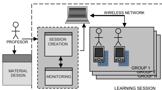
Figure 2. Architectural diagram of the developed tool. The diagram includes the PC and PDAs modules
