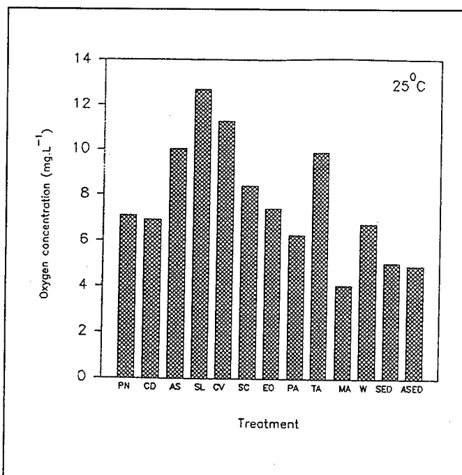
Figure 7. Oxygen concentrations in treated groundwater following 10-day incubation at 25 °C (Single values) (Abbreviations: PN, pondweed; CD, coontail; AS, waterplantain; SL, arrowhead; CV, fox sedge; SC, wool-grass; EO, spikerush; PA, reed canary grass; TA, cat-tail; MA, parrot-feather; W, groundwater; SED, sediment; ASED, autoclaved sediment)
