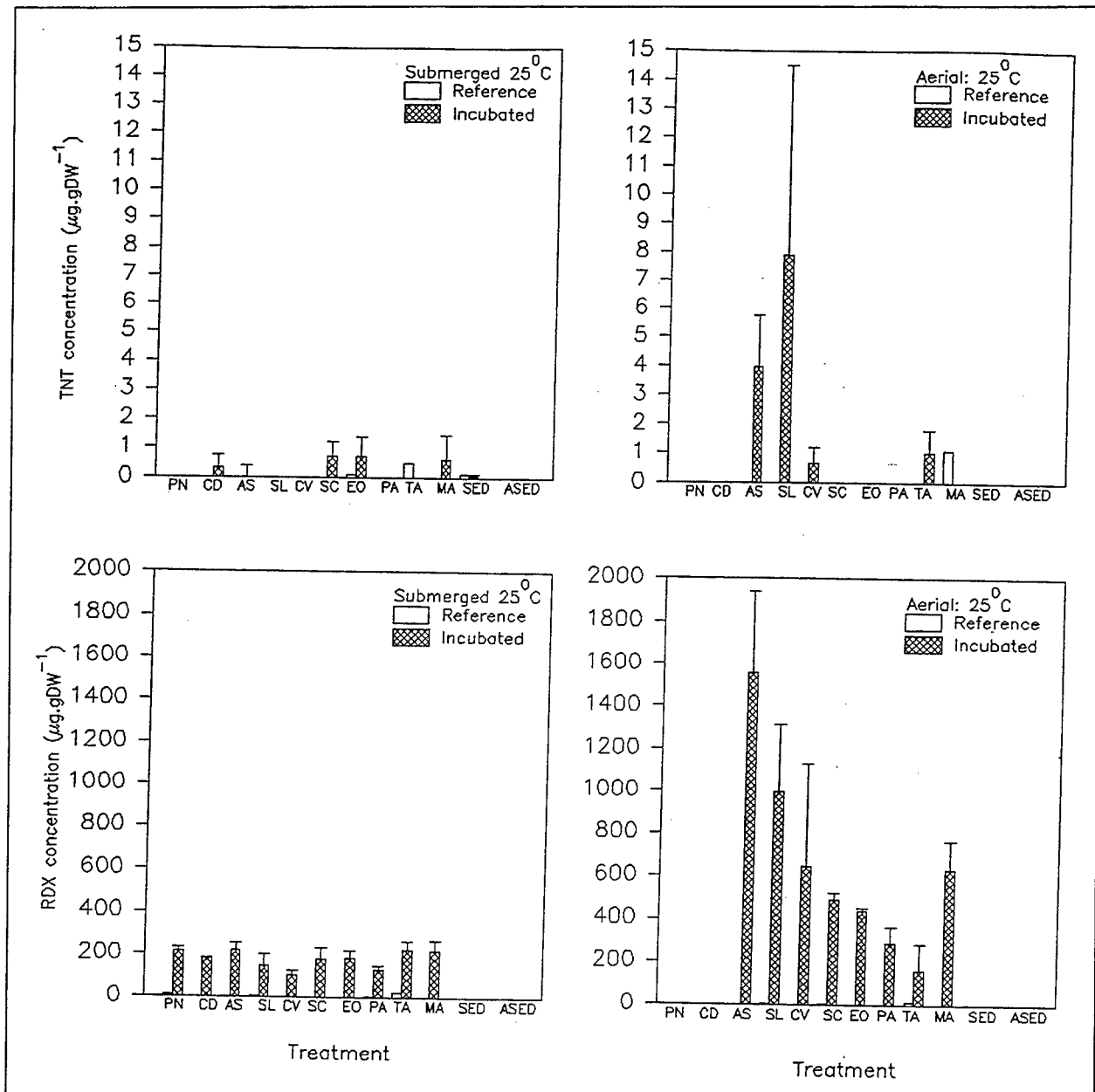
Figure 4. Concentrations of TNT and RDX in aerial and submerged portions of explosives-contacted plants and sediments (mean values of triplicates and standard deviations) and in reference plants (single values), 25 °C incubations (Abbreviations: PN, pondweed; CD, coontail; AS, water-plantain; SL, arrowhead; CV, fox sedge; SC, wool-grass; EO, spikerush; PA, reed canary grass; TA, cat-tail; MA, parrot-feather; SED, sediment; ASED, autoclaved sediment)
