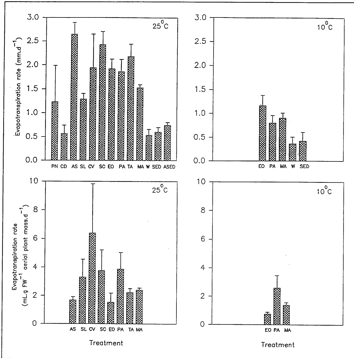
Figure 5. Evapotranspiration rates of groundwater following 10-day incubation (Mean values of triplicates and standard deviations) (Abbreviations: PN, pondweed; CD, coontail; AS, water-plantain; SL, arrowhead; CV, fox sedge; SC, wool-grass; EO, spikerush; PA, reed canary grass; TA, cat-tail; MA, parrot-feather; W, groundwater; SED, sediment; ASED, autoclaved sediment)
