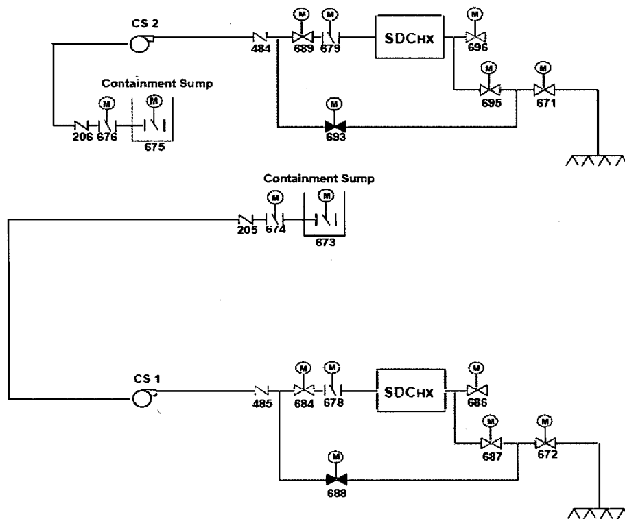
Figure 3-5. Recirculation LOCA, Containment Spray
