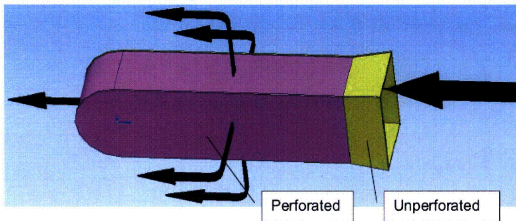
Figure 3-10: CCI Strainer Pocket
