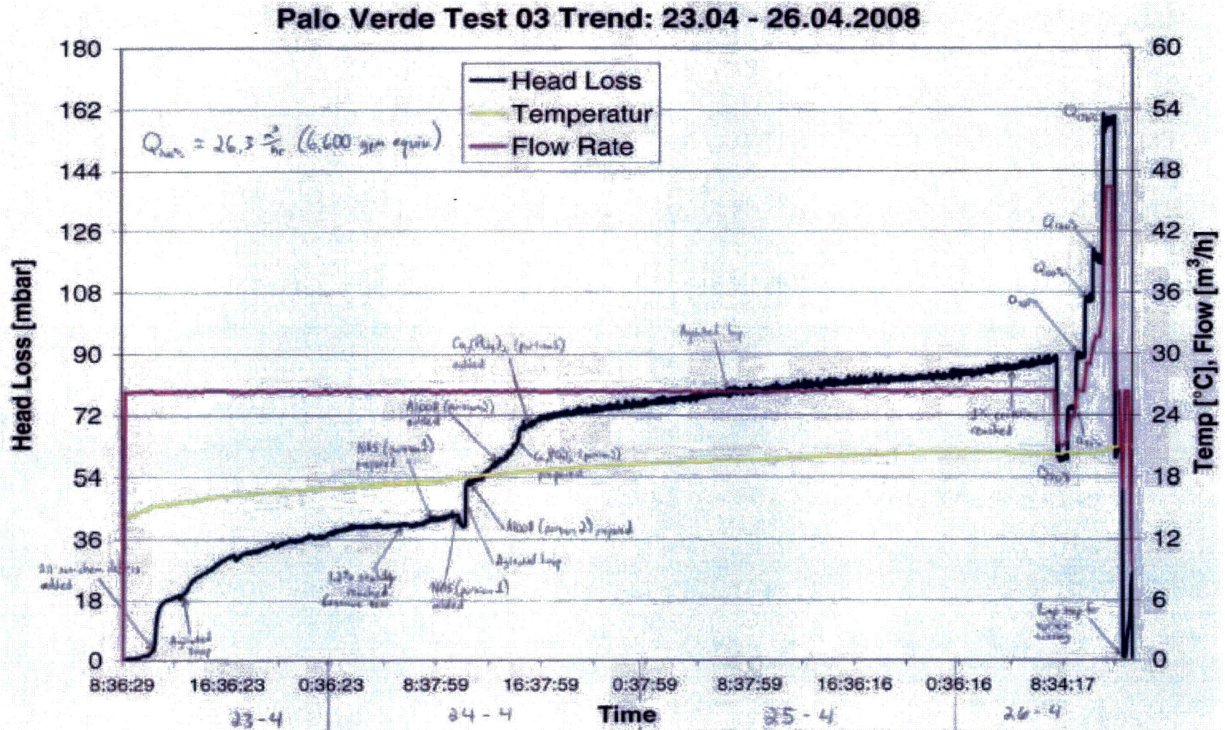
Figure 3-36: Test #3 Chemical Effects Test Plot
