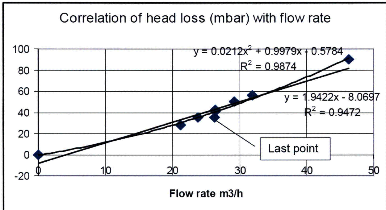
Figure 3-24: Test 2 Flow Sweep Data
