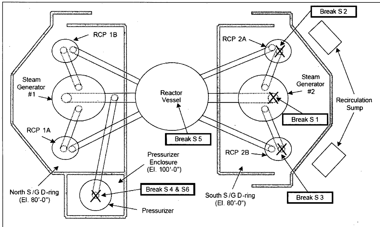
Figure 3-1: Break Locations
