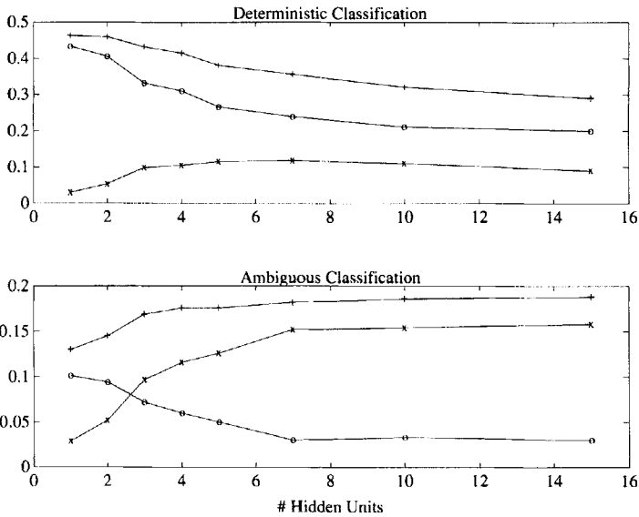
Figure 8: Integrated bias (os), variance ( \times s), and total error (+s) as functions of the number of hidden units in a feedforward neural network.
