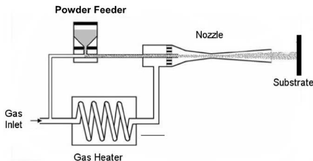
Fig. 1. Schematic of a typical cold-gas dynamic-spray system.
