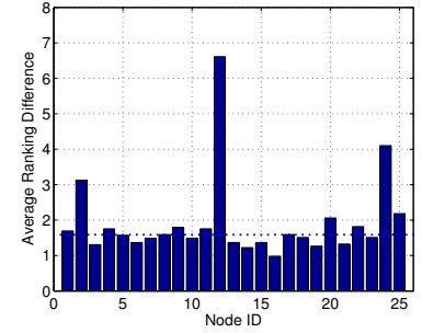
(b) 49 Events
