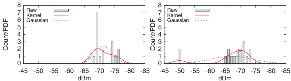
Figure 3. RSSI histograms and their kernel and Gaussian representations, taken from two APs seen in the same bind. The left figure shows how the peaks of a ‘narrow’ bimodal can be more accurately captured by a kernel representation. The right figure shows how a Gaussian can artificially spread out a bimodal that has two distant peaks.
