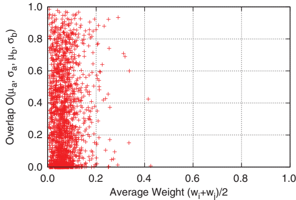
Figure 6. While response rate and received signal strength are moderately correlated (Figure 5), the average weight \frac{w_a+w_b}{2} and overlap O(\cdot) only exhibit very low correlation. In this data set, taken from a nine-story building, the two quantities only have \rho^2=0.11 . This lack of correlation suggests that MAO is, in fact, taking advantage of independent sources of information.
