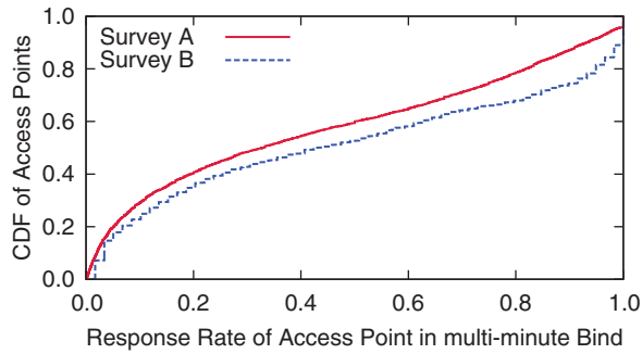
Figure 7. Because response rates range fairly uniformly, penalising equally for the absence of an AP does not appear to be the best use of ‘negative information’. The figure shows the distribution of response rates of access points from binds lasting several minutes from two surveys of the same nine-story building. Survey A was conducted by a commercial location systems provider using their own proprietary equipment and includes 482 binds. Survey B used Nokia N900s and consists of 47 binds. Response rates across these two surveys was similar and in line with other surveys in other locations.
