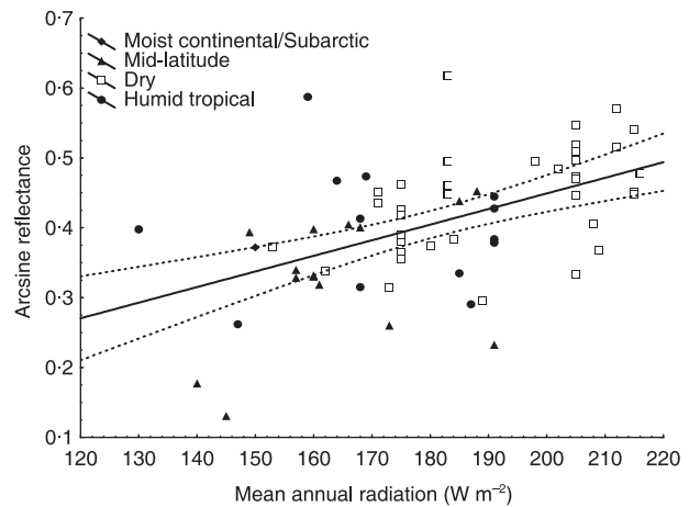
Fig. 2. Interspecific relationship between mean annual radiation (MRAD; \text{W m}^{-2} ) and arcsine square-root transformed skin reflectance ( r ; n = 66 species from 12 families). The ordinary least-square relationship (solid line) is described by the equation: r = 0.002 + 0.002 \times \text{MRAD} ( r^2 = 0.26 , F_{(1,64)} = 22.9 , P < 0.0001 ). Stippled lines indicate 95% confidence intervals. Major climate zones defined according to Bonan (2002) are represented by different symbols.
