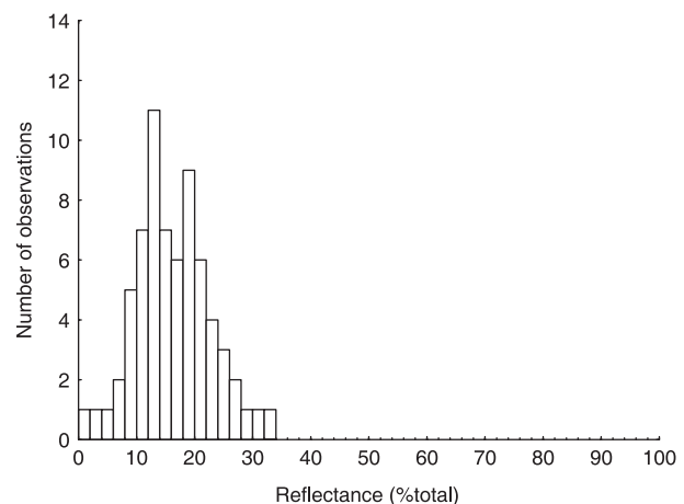
Fig. 1. Frequency distribution of skin reflectance (%) for 68 heliothermic lizard species included in the present study.
