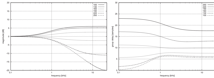
Figure 10: Magnitude and Group Delay responses of the block responsible for head shadowing and ITD ( F_s = 44100Hz ). Azimuth ranging from \theta_{ear} to \theta_{ear} + 150^\circ .
