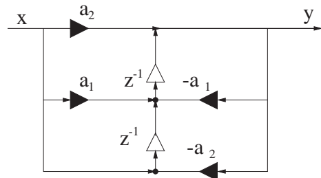
Figure 26: Second-order allpass filter, Transposed Form II
