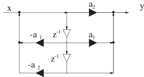
Figure 25: Second-order allpass filter, Direct Form II
