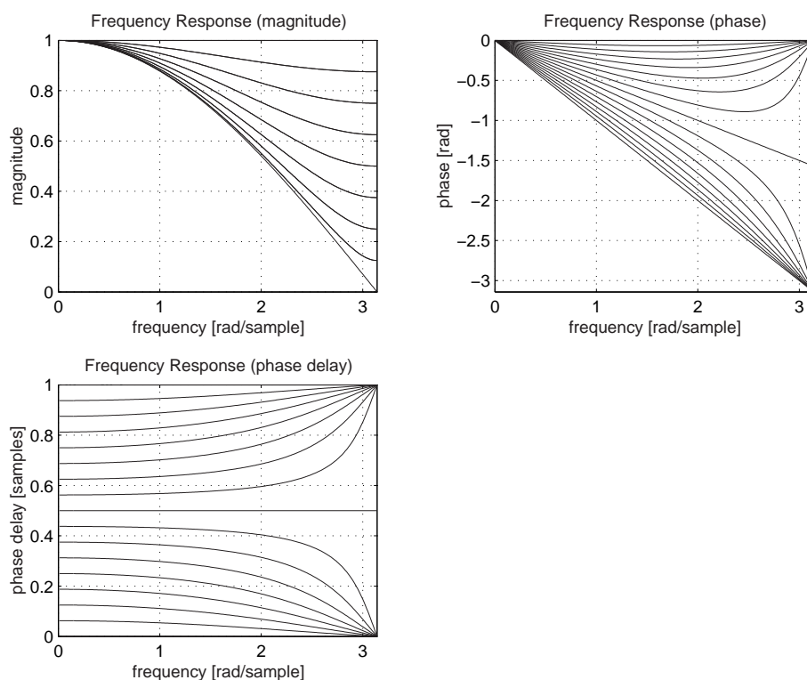
Figure 2: Magnitude, phase, and phase delay responses of a linear interpolation filter (1 - \alpha) + \alpha z^{-1} for \alpha = k/16, k = 0, \dots, 16
