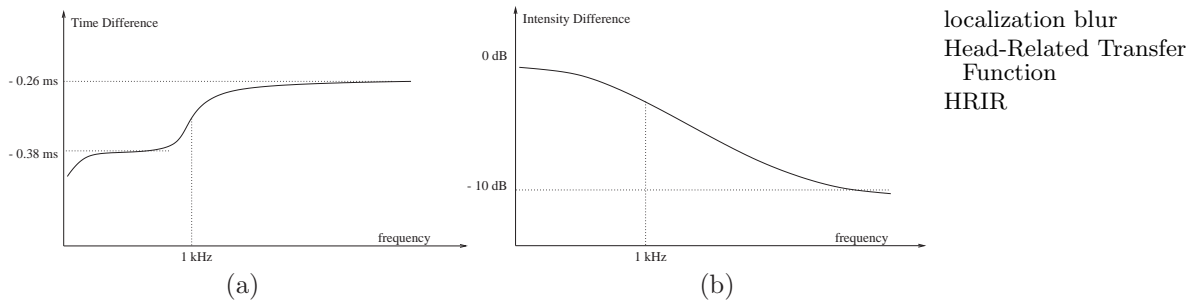
Figure 9: Frequency-dependent interaural time (a) and intensity (b) difference for azimuth 30^\circ .
