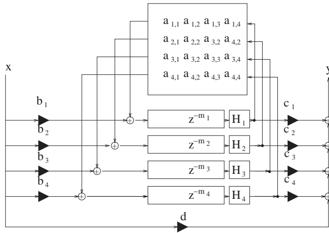
Figure 15: Fourth-order Feedback Delay Network
