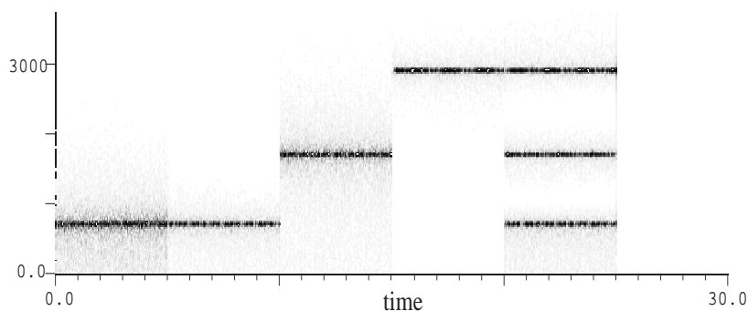
Figure 20: Sonogram of a musical phrase produced by filtering white noise
