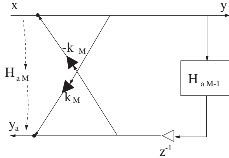
Figure 28: Lattice filter
