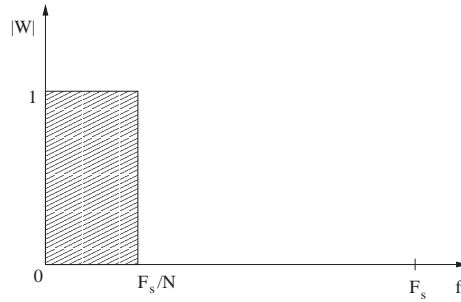
Figure 1: Frequency response of a prototype lowpass filter
