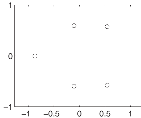
Figure 5: Roots of the polynomial 1 + 2x^2 + 5x^5 in the complex plane
