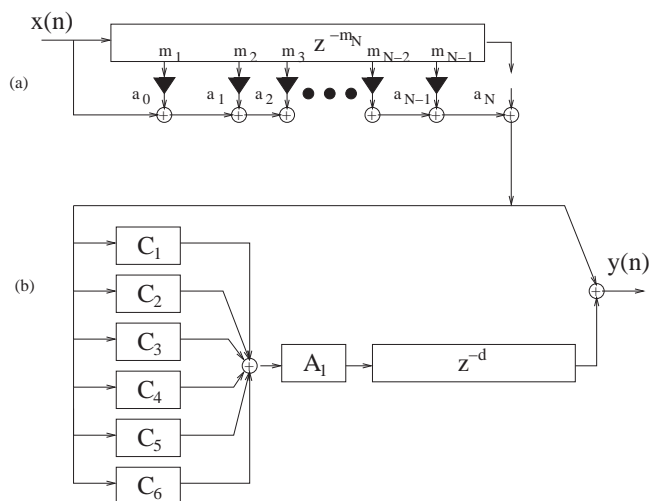
Figure 14: Moorer's reverberator
