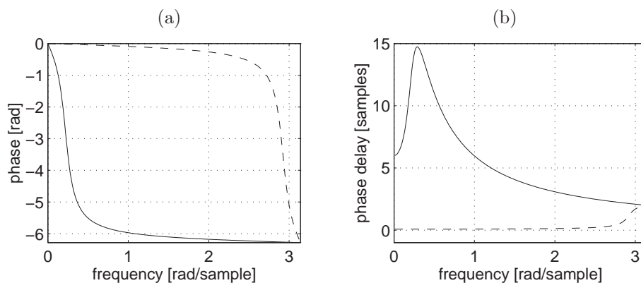
Figure 23: Phase of the frequency response (a) and phase delay (b) for a second-order allpass filter. Poles in p_{1,2} = 0.9 \pm i0.2 (solid line) and p_{1,2} = -0.9 \pm i0.2 (dashed line)
