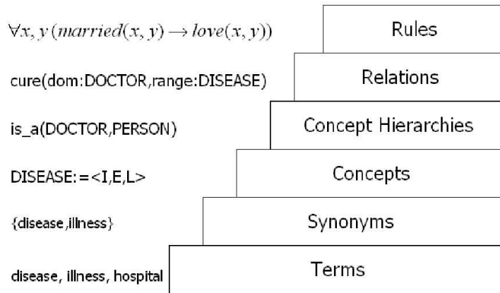
Figure 1. Ontology Learning Layer Cake
