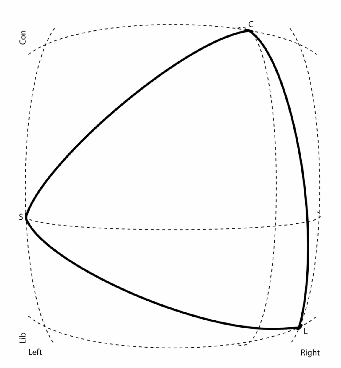
Figure 1.3: Shortest “distances” between actors on a sphere (projected onto a Euclidean plane)
