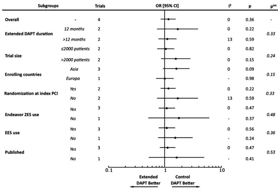
Figure 4 Sensitivity analyses of treatment-effect modification for all-cause death in the subgroups of interest. Odds ratio and (95% confidence interval) are used as summary statistics and are presented as plot: the centre indicates the point estimate and the left and the right ends of the line the (95% CI); I 2 statistic describes heterogeneity across trials included among subgroups of interest, excepting in those cases for which only one trial is included within a subgroup; P int : P-values for interaction between treatment-effect and subgroups are derived with meta-regression analysis. DAPT, dual antiplatelet therapy; PCI, percutaneous coronary intervention; ZES, zotarolimus-eluting stent; EES, everolimus-eluting stent.
