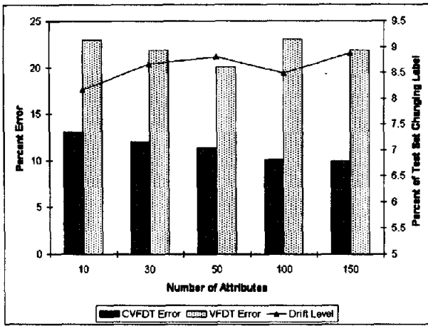
Figure 1: Error rates as a function of the number of attributes.
