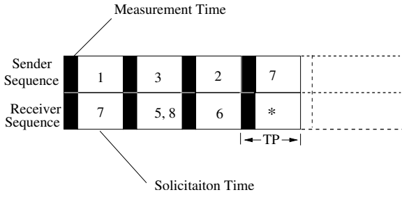
Fig. 2: Sample PV Measurement and Transmission Schedule
