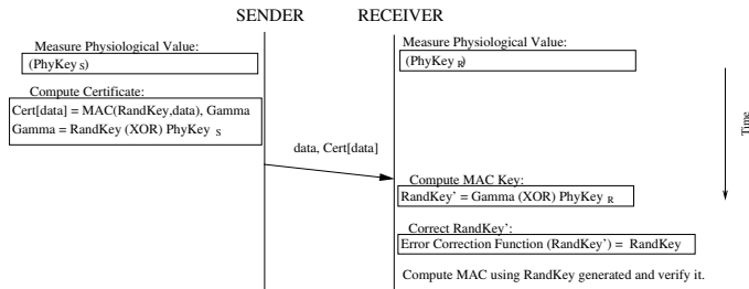
Fig. 1: Using PVs for Authenticated Inter-Sensor Communication
