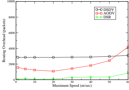
Fig. 13. RPGM (Single Group): Routing Overhead
