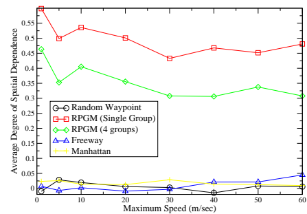
Fig. 3. Average Degree of Spatial Dependence
