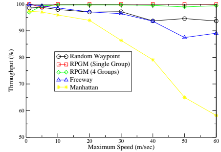
Fig. 5. DSR Throughput
