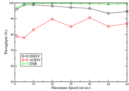
Fig. 9. RPGM (4 Groups): Throughput
