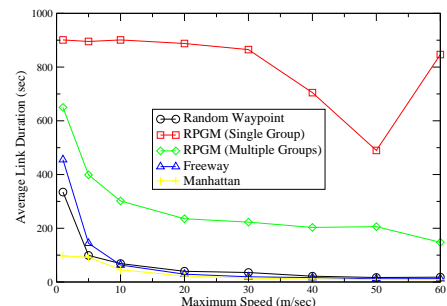
Fig. 4. Average Link Duration
