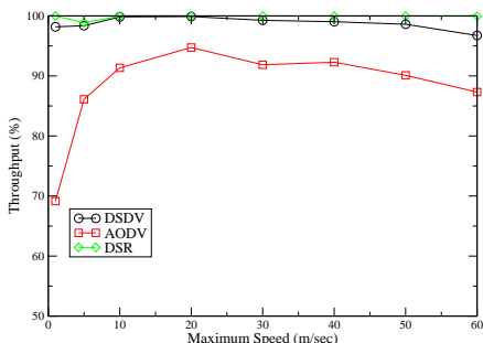
Fig. 8. RPGM (Single Group): Throughput
