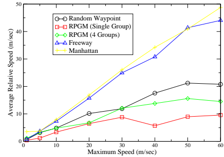
Fig. 2. Average Relative Speed
