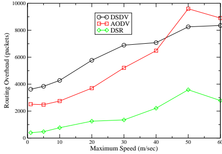
Fig. 14. RPGM (4 Groups): Routing Overhead
