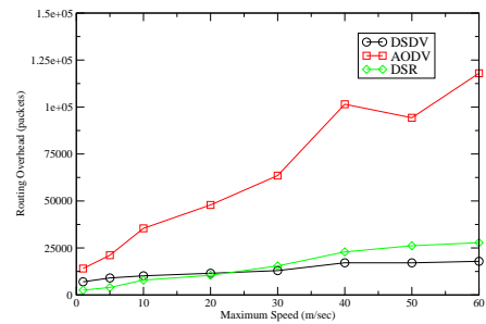
Fig. 12. Random Waypoint: Routing Overhead
