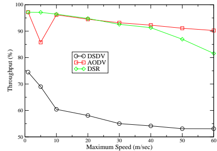
Fig. 11. Manhattan: Throughput
