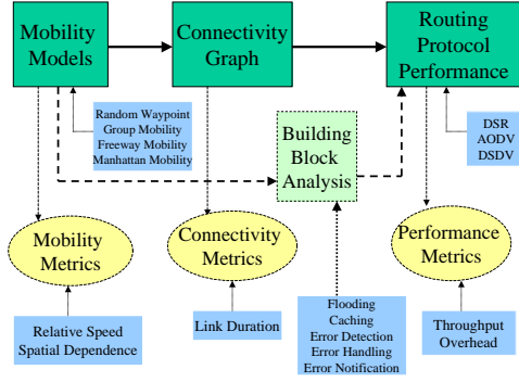
Fig. 1. IMPORTANT Framework
