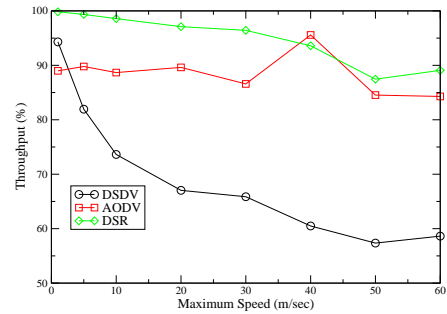
Fig. 10. Freeway: Throughput
