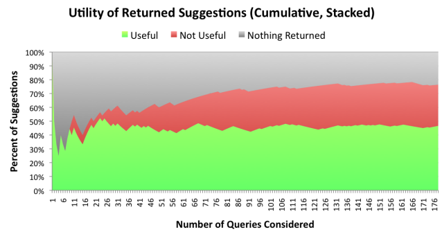
Figure 9. Relative utility of returned suggestions for queries issued during the Processing workshops.
