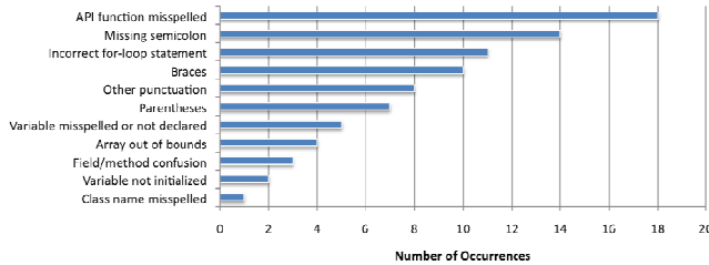
Figure 11. Error types for queries that yielded useful suggestions from HelpMeOut.
