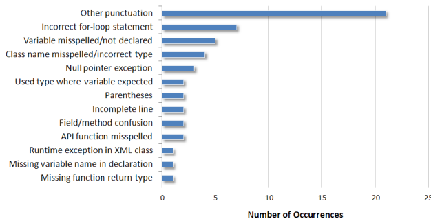
Figure 12. Error types for queries that yielded suggestions, but where suggestions were not useful.
