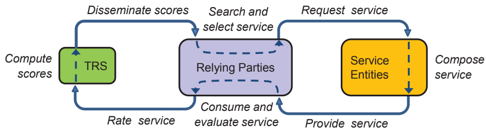
Fig. 1. Functional integration of Trust and Reputation Systems
