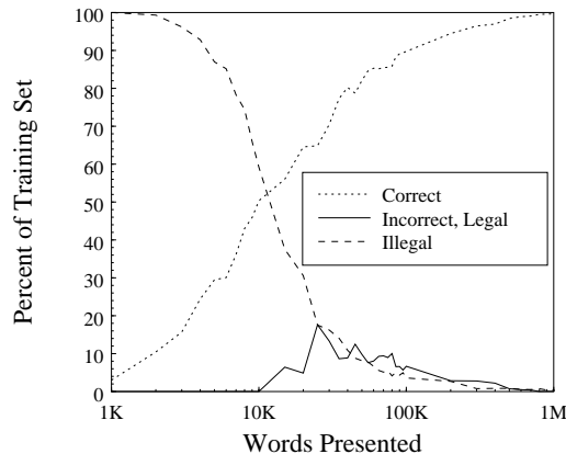
Figure 4. Pattern retention accuracy over the course of phonological training.
