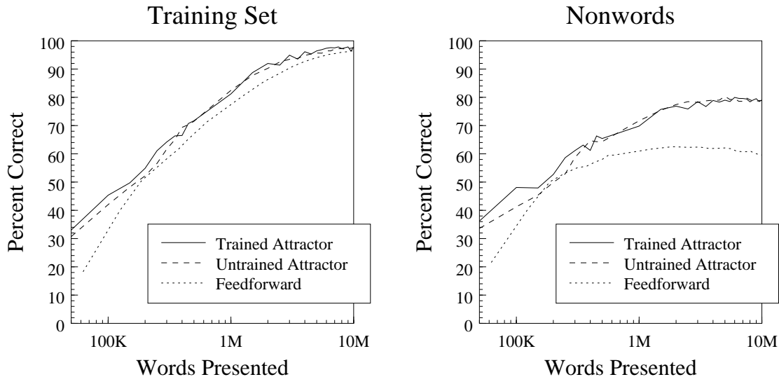
Figure 10. Comparison between the normal reading model, the feedforward model, and the initially untrained attractor model on the training set (left) and nonword generalization (right).
