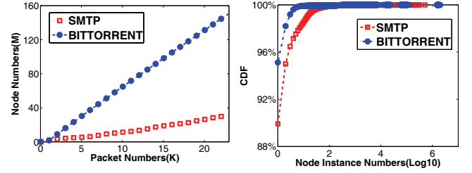
(a) Node space size versus number of processed packets (b) CDF of node frequency
