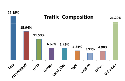
Fig. 9: Protocols composition in hybrid traffic trace.
