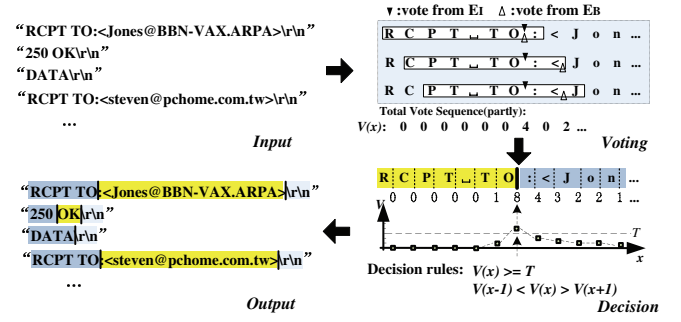
Fig. 1: Overview of the VE algorithm.
