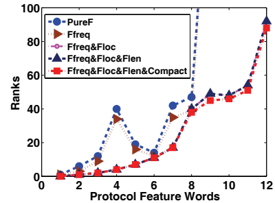
Fig. 7: Comparison of different combinations of score functions in the ranking model.
