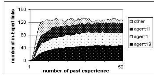
Figure 6. In-link distribution
