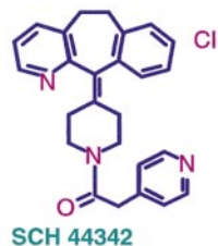
Fig 3. Structures of representative agents from different classes of F1ase inhibitors.
