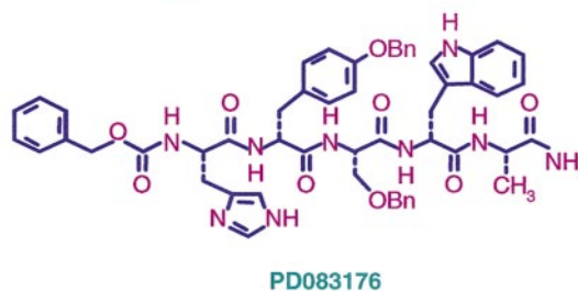
Fig 3. Structures of representative agents from different classes of F1ase inhibitors.
