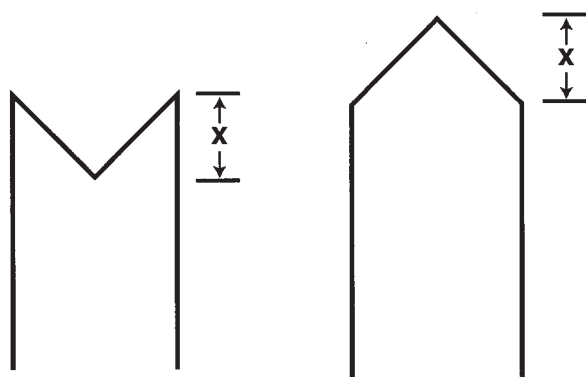
FIG. 18. Antibody shapes described by a real number, for example, the height ( +x ) or depth of the antibody binding site ( -x ), in continuous shape space.
