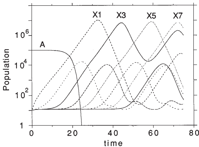
FIG. 23. Dynamics of a network undergoing percolation. The parameters are k=10^{-5} , A_0=10^5 , d=1.0 , p=1.5 , z=3 , m=10 , \theta_1=300 , and \theta_2=10^6 . From Neumann and Weisbuch, 1992a, reproduced with permission.
