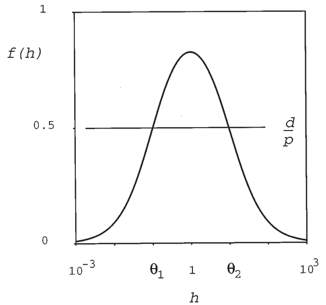
FIG. 12. The log-bell-shaped activation function f(h) defined by Eq. (4.3). As discussed in the text, when m is small, intersections of the line y = d/p with the bell-shaped curve define the activating and suppressive field values, L and H , respectively. For the parameters used here, p = 1 and d = 0.5 , these intersections occur near the field values \theta_1 and \theta_2 .
