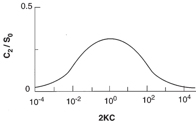
FIG. 7. A plot of the equilibrium nondimensional concentration of cross links ( C_2/S_0 ) vs \log(2KC) . The curve has a single peak at 2KC=1 , about which it is symmetric. Since the surface concentration of receptor sites is S_0 and each cross link occupies two sites, C_2/S_0 \leq 0.5 .
