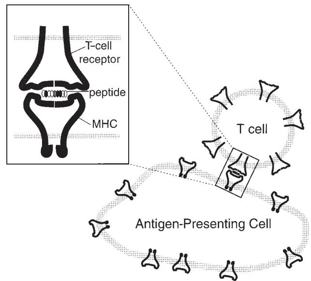
FIG. 3. T cells, via their T-cell receptor, recognize MHC-peptide complexes on the surface of antigen-presenting cells.
