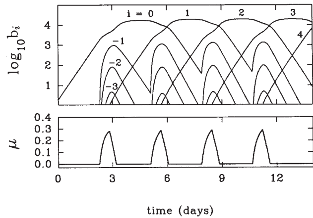
FIG. 9. The lower panel shows the optimal mutation schedule that generated the dynamics in the upper panel. There are a number of rounds of mutation, each of which produces some cells that have a one-step increase in their affinity class. After an advantageous mutant appears, mutation is turned off to maximize the growth of the mutant clone and to prevent its loss through further mutation. The upper panel shows the dynamics of the B-cell response, b_i vs t . The response begins with a single B-cell clone in affinity class i=0 . Mutation, when turned on, generates cells in lower affinity classes ( i=-1, -2, -3 , as well as cells in higher affinity classes ( i=1, 2, 3, 4 ).
