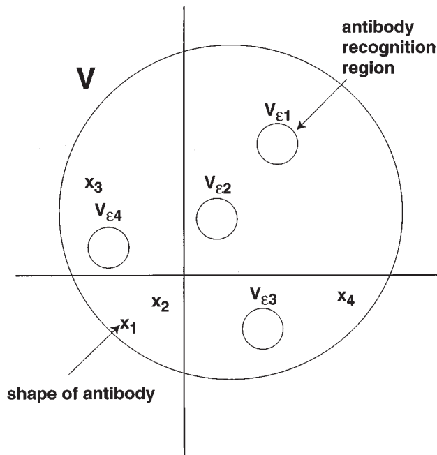
FIG. 5. Diagrammatic representation of shape space. Antibody of shape x_i recognizes those epitopes whose shapes lie within a region of shape space, of volume V_{\epsilon_i} , called a “recognition ball” or “recognition region.” The entire shape space is assumed to be a bounded region of R^n with volume V .
