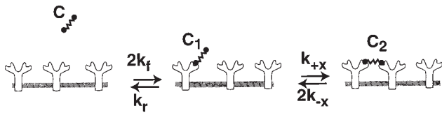
FIG. 6. Bivalent ligand in solution at concentration C reacts with bivalent surface receptors. The forward and reverse rate constants for the binding of a single site on the ligand to a single receptor site are k_f and k_r , respectively. Once the ligand is bound to the surface at one site, with concentration C_1 , its second site can bind to another receptor site with forward and reverse rate constants k_x and k_{-x} , respectively, to form a doubly bound ligand C_2 . Note that the second reaction, the “cross-linking step,” is a surface reaction, whereas the first reaction involves the binding from bulk solution. Thus k_f and k_x have different units and need to be distinguished.
