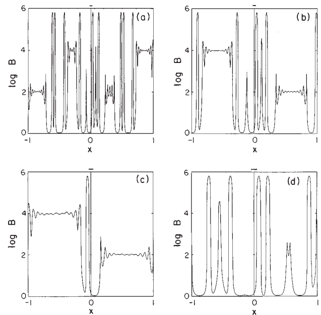
FIG. 32. The equilibrium distributions of B-cell populations as a function of the range of interaction in shape space. The interaction range is indicated by the heavy horizontal line at the top of each panel. See De Boer, Segel, and Perelson (1992) for details.
