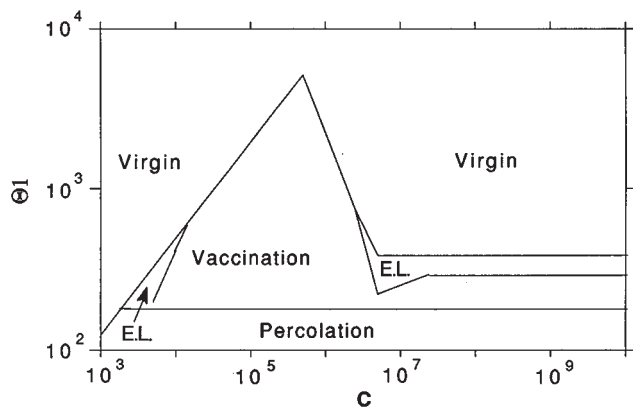
FIG. 22. Phase diagram derived from the window-automaton model [defined by Eq. (4.17)]. \theta_1 is the excitation threshold and C is related to the antigen elimination time [see Eq. (4.22)]. The transition from virginity to excitation is different for the three regimes of C . The transition from percolation to vaccination is independent of C . Two extended-localization regimes, denoted E.L., are observed. This diagram corresponds to a relatively low initial antigen concentration, A_0 = \sqrt{\theta_1 \theta_2} . (A large initial antigen concentration, which can result in tolerance, would further complicate this phase diagram.) From Neumann and Weisbuch, 1992a, reproduced with permission.
