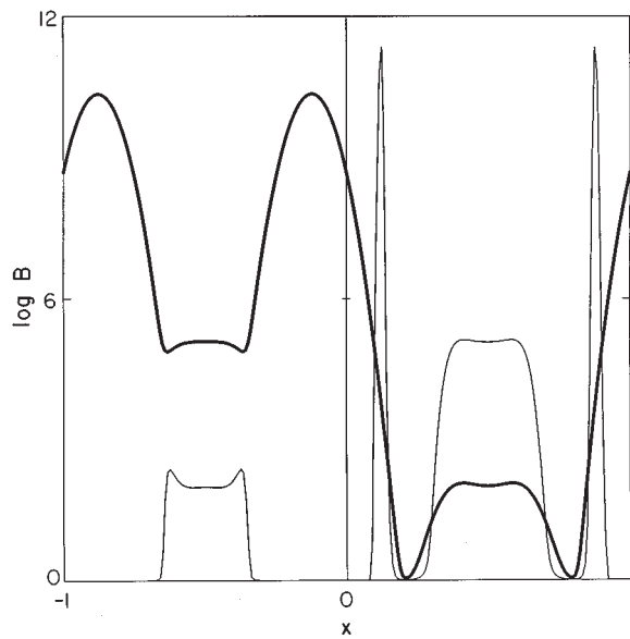
FIG. 31. Pattern formed in a continuous one-dimensional shape space by an AB model. Here x , the shape variable, is the horizontal axis. We show the distribution of the B-cell population (light lines) and of the field (heavy lines) attained long after a destabilizing perturbation of the suppressed state. The B-cell population, which is plotted on a logarithmic scale ranging to 10^{12} , exhibits two unrealistically large peaks, which are sustained by self-stimulation. In addition one sees a region for 0.2 < x < 0.6 where the population is in the immune state, and a complementary region in the negative part of shape space in which the population is suppressed.
