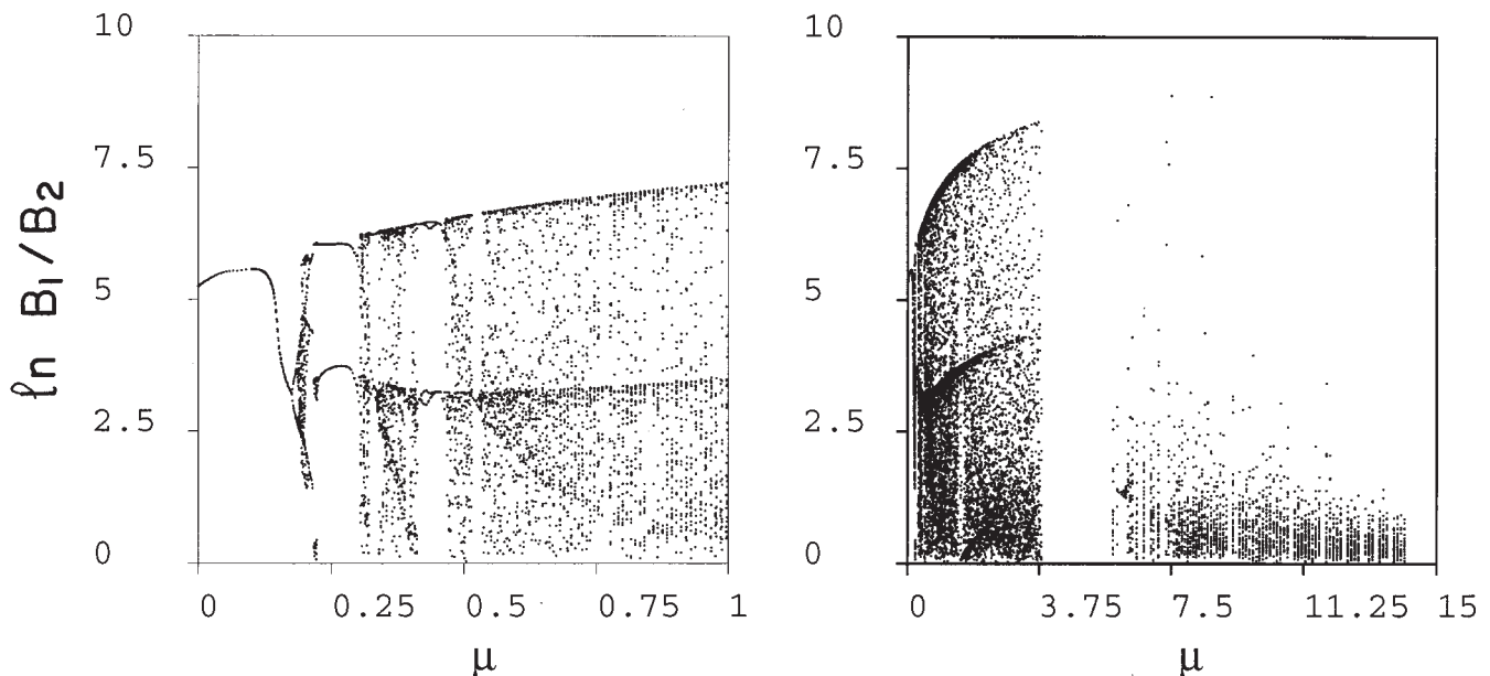
FIG. 30. Dynamics of the AB model as seen by trajectories going through the Poincaré section defined by A_1 - A_2 = 0 . The behavior of the model is either stationary, periodic, or apparently chaotic, depending upon the value of \mu .
