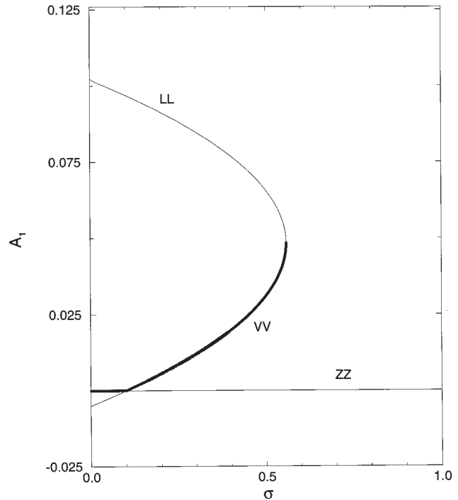
FIG. 28. Bifurcation diagram of AB model. Here the nondimensional source \sigma is varied and the equilibrium concentration of antibody A_1 plotted. For low values of \sigma the virgin state with low amounts of antibody present, the VV state, is negative, and only the ZZ virgin state with no antibody present is a physically realizable solution to the AB model equations. The dark line indicates a stable steady state. For \sigma > 0.1 , the ZZ state is unstable and the VV state is the virgin state for this system. For values of \sigma > 0.56 this system has no virgin state.
