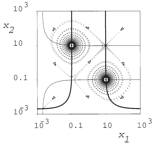
FIG. 15. Phase portrait of the dynamics of two interacting clones. Of the five singular points in the plane, only the virgin state (x_1, x_2) = (L, L) , the tolerant state (x_1, x_2) = (H, L) , and the immune state (x_1, x_2) = (L, H) are attractors. The two symmetric states (L, L) and (H, H) are unstable.
