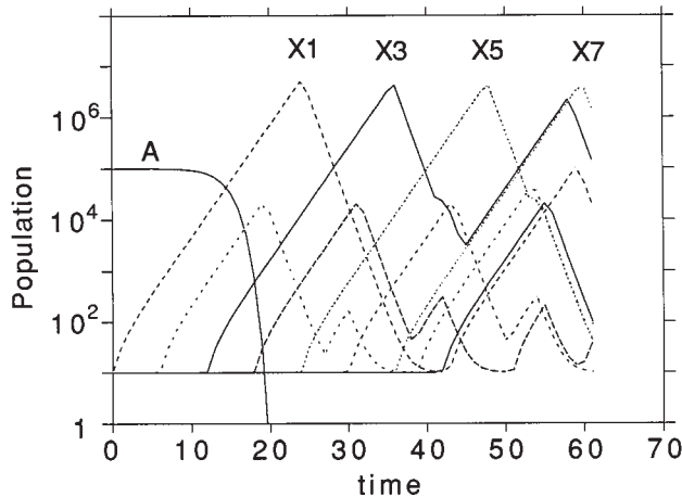
FIG. 25. Dynamics of a network undergoing percolation predicted with the window-automaton model. The dynamics are very similar to those illustrated in Fig. 23 for the log-bell-shaped proliferation function, apart from a slight difference in time scales. The same parameters were used in both simulations: k = 10^{-5} , A_0 = 10^5 , d = 1.0 , p = 1.5 , z = 3 , m = 10 , \theta_1 = 300 , and \theta_2 = 10^6 . From Neumann and Weisbuch, 1992a, reproduced with permission.
