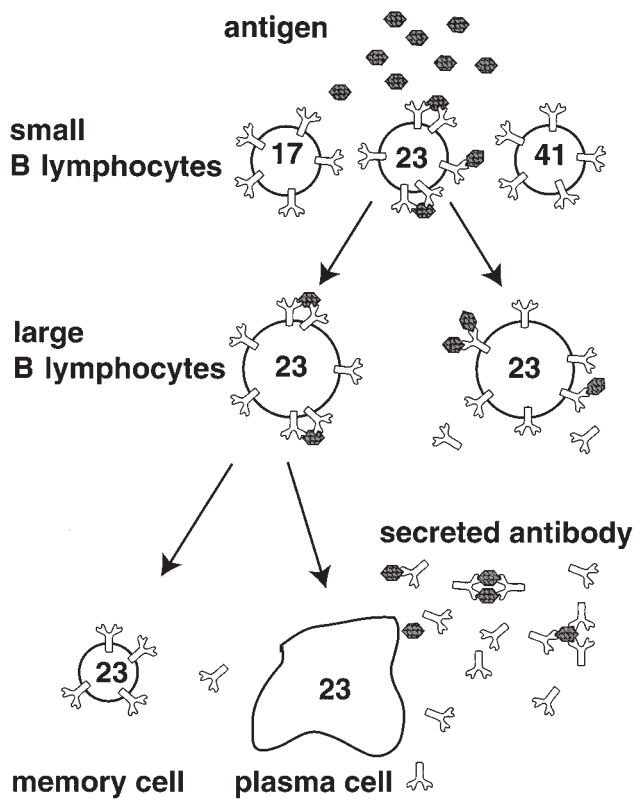
FIG. 4. Clonal selection. Small resting B cells created in the bone marrow each carry a different receptor type defined by their V_H and V_L regions (see Fig. 1). Here B cells are labeled by their receptor type. B cells of type 23 recognize the antigen and become large lymphocytes, which proliferate and differentiate into antibody-secreting cells and memory cells. The most differentiated antibody-secreting cell is a plasma cell.
