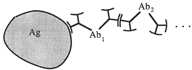
FIG. 11. Jerne idiotypic cascade. The antigen Ag is recognized by B cells, which secrete antibodies Ab_1 . These antibodies are themselves recognized by “anti-idiotypic” B cells, which secrete antibodies Ab_2 . Further interactions can lead to Ab_3 antibodies that recognize Ab_2 and so on.
