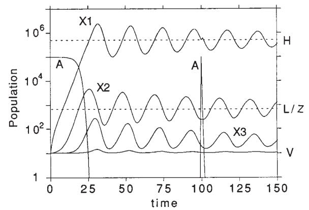
FIG. 20. Dynamics of an immune response generated by a network with a Cayley tree topology when antigen A , recognized by a clone at level 1, x_1 , is injected into a system in the virgin state. The response causes the system to approach the immune attractor. In the immune configuration the largest population is localized at the first level. x_1 is high ( H ) and is sustained by interacting with x_2 , which is at an intermediate population level ( L/z ). In a network with a Cayley tree topology, where z is the number of clones connected to any clone, one sees that clones x_3 as well as the rest of the clones in the network are virgin ( V ) (or almost virgin) after the system settles into this attractor. When antigen is presented again, it is eliminated faster than the first time. Simulation parameters were as follows: k=10^{-6} , A_0=5000 , d=0.5 , p=1 , z=3 , m=10^{-3} , \theta_1=2000 , and \theta_2=10^5 . From Neumann and Weisbuch, 1992a, reproduced with permission.
