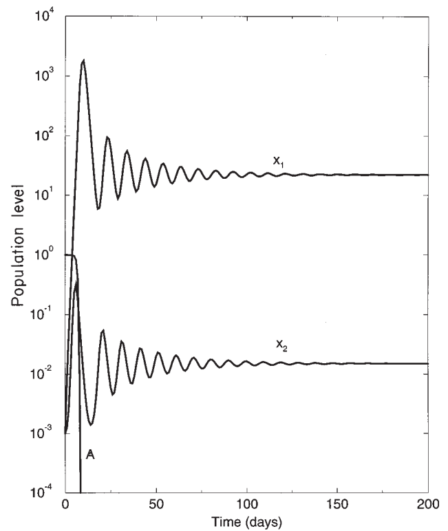
FIG. 13. Dynamics of a response induced by injecting antigen A that results in the system's approaching the immune attractor. The clone population sizes are plotted vs time in days. In the immune configuration the largest population is localized at the first level. x_1 is high ( H ) and is sustained by interacting with x_2 , which is at a lower level ( L ).
