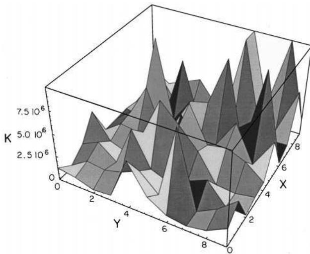
FIG. 8. A random landscape. The affinity of an antibody depends on its variable region. However, one cannot yet predict affinity from sequence. If affinities are assigned to variable-region gene sequences at random, say from a log-normal distribution, then a random landscape results. Here a two-dimensional representation of sequence space is indicated, the x and y coordinates being arbitrary indexes. Each integer value (x,y) indicates a sequence, above which a random affinity K(x,y) is plotted.
