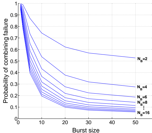
Figure 4: The upper bound on p_f as a function of the burst size, b . From top to bottom, the curves are plotted for the span of values of number of blocks, N_B = 2, 4, 6, 8, 10, 12, 14 and 16 .
