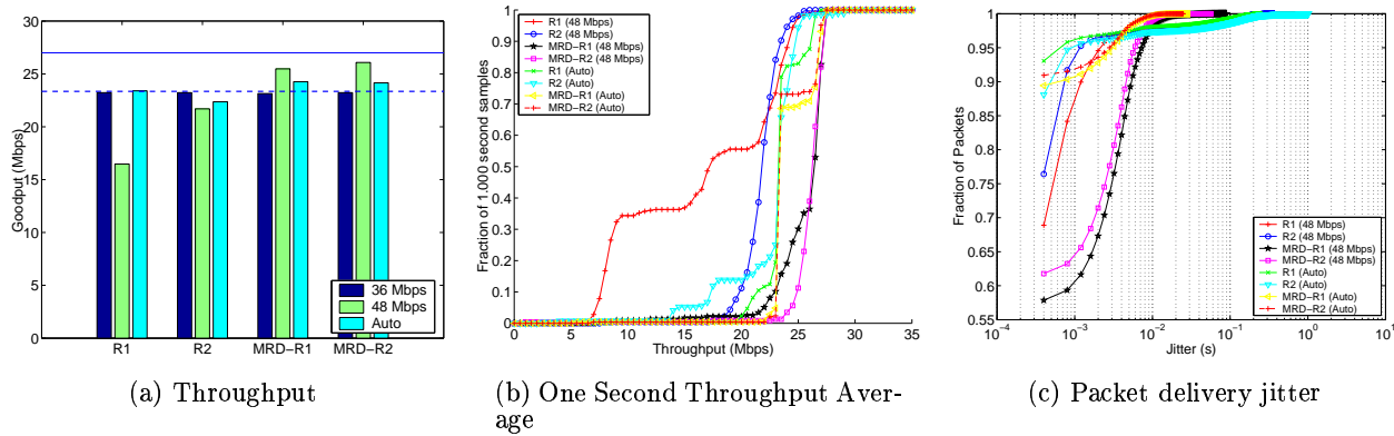
Figure 12: Static Experiment Analysis. Left: Throughput averaged over 5 trials. The dashed line marks the maximum achievable UDP throughput (23 and 27 Mbps) for 802.11a fixed at 36 Mbps and 48 Mbps bit-rates. Center: Distribution of throughput averaged in non-overlapping one-second window samples. Right: Delay jitter above the minimum one-way packet delivery time.
