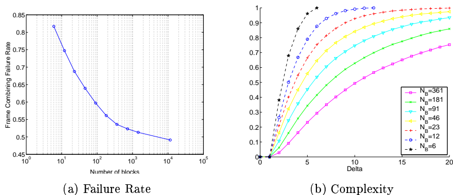
Figure 10: Trace-driven simulation of p_f and \Delta at various N_B .
