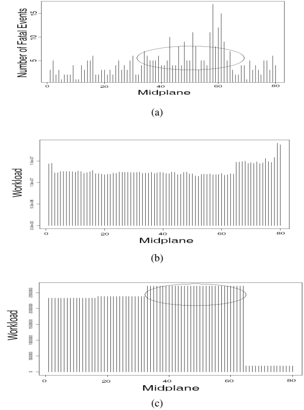
Figure 4: (a) Number of fatal events on each midplane, (b) workload on each midplane, and (c) workload of wider jobs, (i.e., the job requesting no less than 32 midplanes) on each midplane. In (a) and (c), we highlight midplane 33–64 to present the impact of wider jobs on failure rate.
