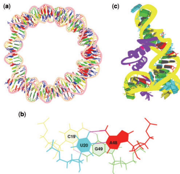
Figure 3. Examples of the unique representations of nucleic acid structures available through the w3DNA server. (a) Color-coded composite block/backbone/tube representation of the DNA in the currently best-resolved nucleosome core-particle structure (31) (PDB ID: 1KX5). (b) Stacking diagram illustrating the overlap and hydrogen-bonding patterns of adjacent base pairs (C 19 -G 49 and U 20 -A 48 ) in model 1 from the ensemble of NMR structures of the complex of a 55 nucleotide fragment of X. laevis 5S rRNA with three zinc fingers of transcription factor TFIIIA (32) (PDB ID: 2HGH). (c) Schematic 'NMR-ensemble' image of the bases, RNA backbones, and protein ribbons in 15 of the 20 models of the aforementioned RNA-protein complex (32). Color coding identical to that in Figure 2, save for the depiction of U in aqua.
