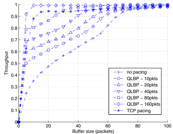
Fig. 11. Link utilization v.s. various buffer size
