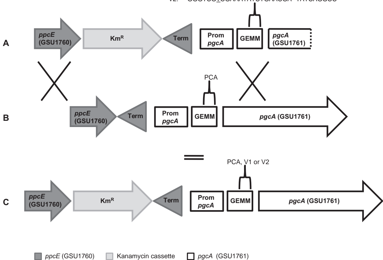
Fig. 3. Introduction of mutations found in V1 and V2 pgcA GEMM riboswitches into G. sulfurreducens PCA chromosome. A kanamycin cassette was included in the middle of PCR constructs (A) containing in 5' the complete PCA ppcE gene and in 3', PCA, V1 or V2 ppcE rho-independent terminator (Term), pgcA promoter region (Prom), pgcA GEMM riboswitch and the beginning of pgcA coding sequence. The base pair inserted in V1 pgcA GEMM riboswitch is in italic whereas the transition found in V2 pgcA GEMM riboswitch is underlined. Following electroporation, the linear PCR constructs were incorporated by homologous recombination in PCA chromosome (B). This process results in three strains containing a kanamycin cassette and either the PCA, V1 or V2 pgcA GEMM riboswitch sequence (C).
