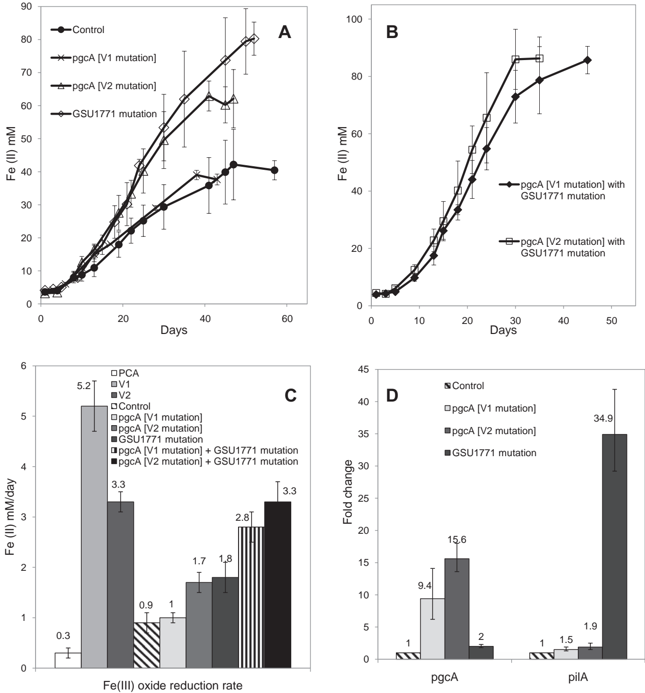
Fig. 4. Fe(III) oxide reduction and gene expression in strains mimicking strains V1 and V2. All strains contain the kanamycin cassette upstream of GSU1761 that is present in the control strain. Fe(III) oxide reduction in control strain and strains with single mutations (A) or in double mutants (B). Each curve is the mean of at least three independent Fe(III) oxide reduction experiments. Summary of Fe(III) oxide reduction rates of all strains in this study (C). Impact of mutations on expression of pgcA and pilA measured by qRT-PCR compared to the control strain during growth on Fe(III) citrate (D). The qRT-PCR results are from at least three replicates for each strain.
