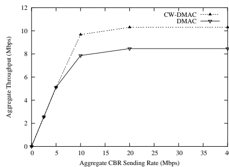
Figure 9. Aggregate throughput in a 30 node random topology.
