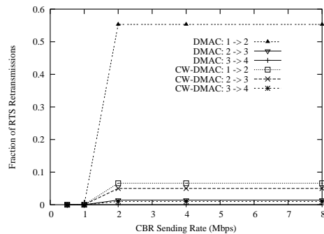
Figure 8. RTS Retransmission in a linear topology.
