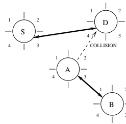
Figure 2. Directional hidden terminal problem due to unheard RTS/CTS.
