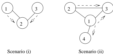
Figure 4. Simple scenarios to study deafness and directional hidden terminal problems.
