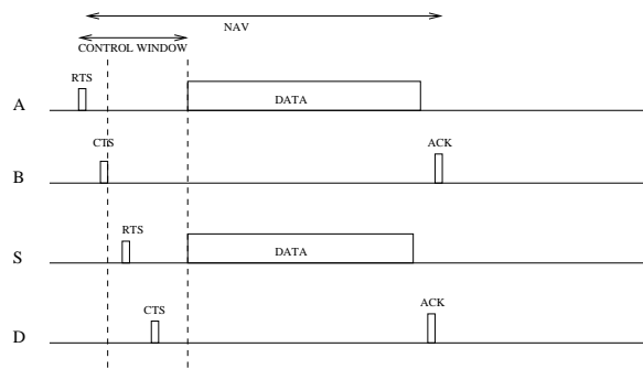
Figure 3. Control window mechanism to prevent directional hidden terminal problem
