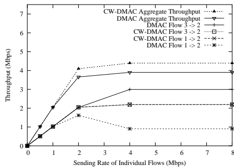
Figure 6. Throughput of different flows in scenario (i). The curves for CW-DMAC Flow 3 \rightarrow 2 and CW-DMAC Flow 1 \rightarrow 2 overlap.
