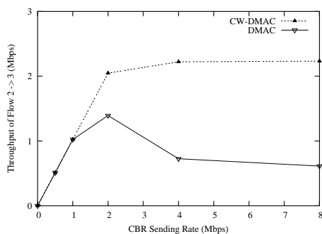
Figure 7. Throughput of flow from node 2 to node 3 in scenario (ii).
