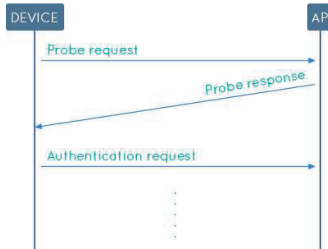
Fig. 14. This figure visualizes the communication between a device and an access point, using probing.
