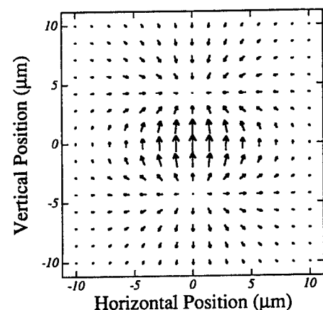
Fig. 1. The dc electric field produced from the charge distribution given by Eq. (2) below. With this dc field shape we successfully predicted the results of six experiments.
