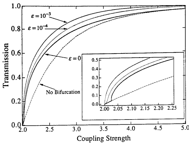
Fig. 6. Calculated transmission (throughput) of a mutually pumped phase conjugator with no bifurcation (i.e., the one-region geometry of Fig. 3a) and with one bifurcation (i.e., the three-region geometry of Fig. 3b) versus coupling coefficient G , for equal-intensity incident beams put into the device ( q = 1 ). The bifurcated data correspond to seeding values of \epsilon of 0, 10^{-4} , and 10^{-3} . The inset shows the region near threshold.
