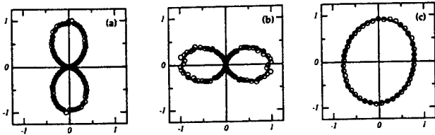
FIG. 4. Polar maps of the measured (circles) and predicted (solid lines) dc electric field strength at the center of Figs. 1, 2, and 3. (a) In case 1 the field is completely along \hat{y} . (b) In case 2 the field is completely along \hat{x} . (c) In case 3 the dc field spirals with z .
