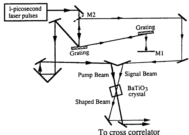
Fig. 1. Experimental setup for measuring pulse-shape changes caused by two-beam coupling in a photorefractive crystal. The signal pulse was first broadened by a factor of 12 using a grating pair and then made to intersect a strong pump pulse in a BaTiO 3 crystal. Mirror M1 was tilted slightly downward to deflect the backward-going beam slightly below the forward-going beam, where it could be picked off by mirror M2. The shape of the signal pulse was measured by using cross correlation in a second-harmonic-generating crystal.
