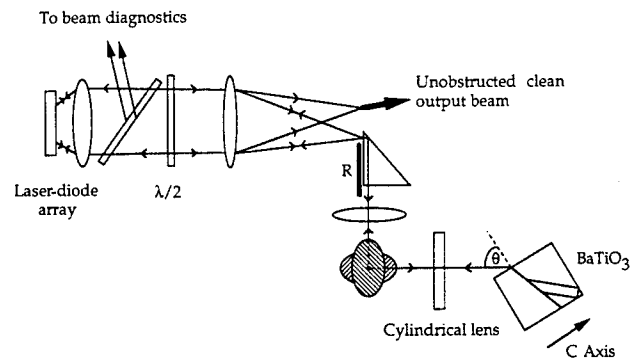
Fig. 1. Laser-diode array coupled to a self-pumped phase conjugator. The half-wave plate rotates the plane of polarization, and the two 45° mirrors align the coherence plane and the plane of polarization parallel to the BaTiO 3 crystal's c axis. The right-angled prism and the vertical razor edge R form an adjustable aperture in the far field. The angle of incidence of the signal beam on the crystal is \theta = 60^\circ .
