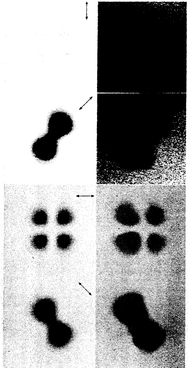
Fig. 4. Photographs of the observed and predicted far-field mode patterns. We oriented the analyzing polarizer horizontally and photographed the far-field pattern of generated green light. The arrow indicates the reading beam's polarization.
