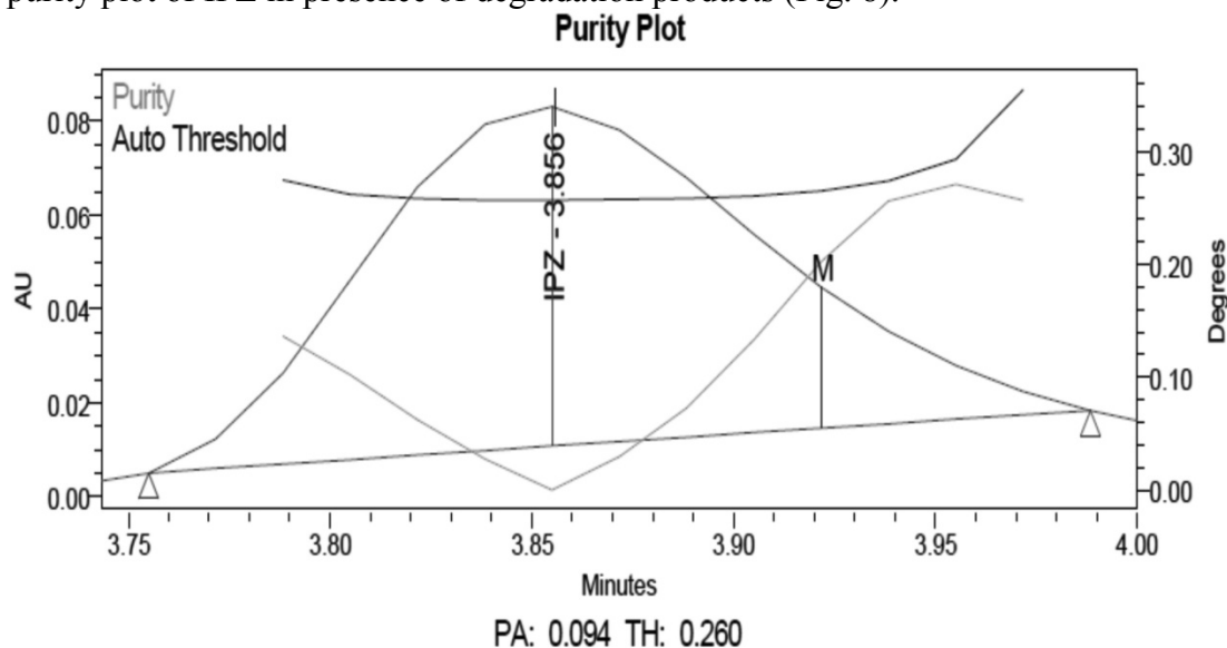
Fig. 8: Purity Plot of Ilaprazole
