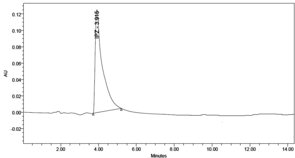
Fig. 6: HPLC chromatograms of Photolytic degradation of IPZ
