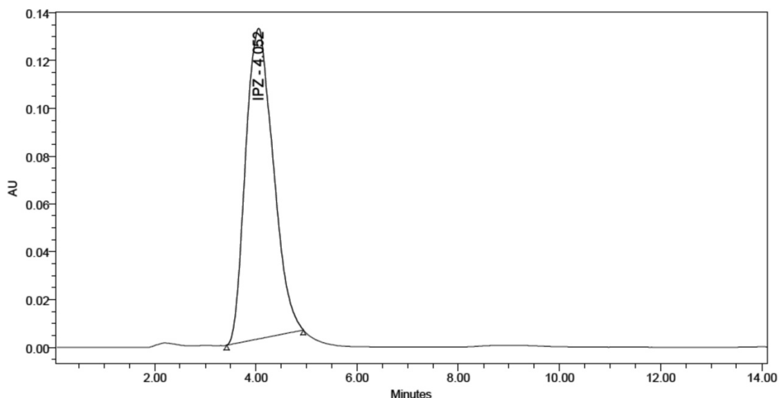
Fig. 4: HPLC chromatograms of Alkali Hydrolysis degraded IPZ
