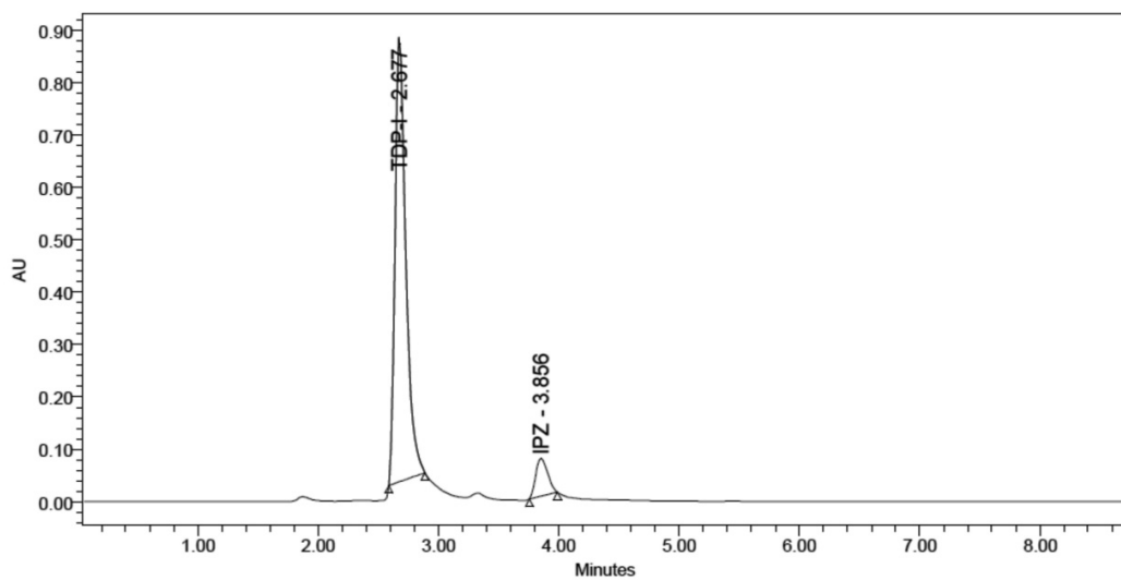
Fig. 7: HPLC chromatograms of Thermal degradation of IPZ
