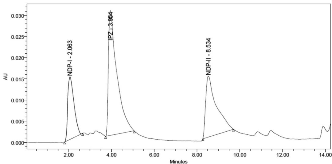
Fig. 2: HPLC chromatograms of Neutral hydrolysis degraded IPZ
