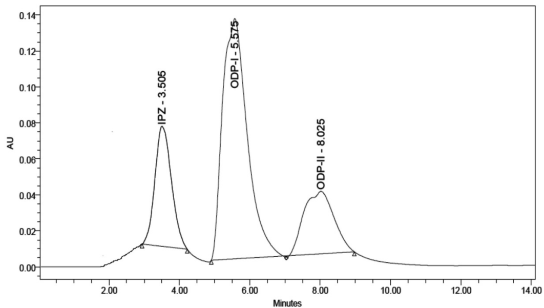
Fig. 5: HPLC chromatograms of Oxidative degradation of IPZ
