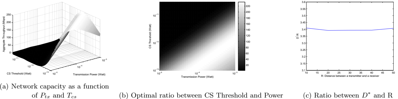
Figure 2: Existence of optimal carrier sense range.
