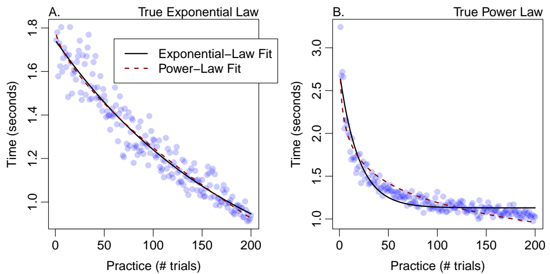
Figure 8: Mean task completion time as a function of practice for simulated data. Means are averages over 30 participants. Solid and dashed lines show best least-squares fit for three parameter exponential and power laws, respectively. A. Each individual’s data follow an exponential law and were generated with \mathcal{M}_e in (26). B. Each individual’s data followed a power law and were generated with \mathcal{M}_p in (27).
