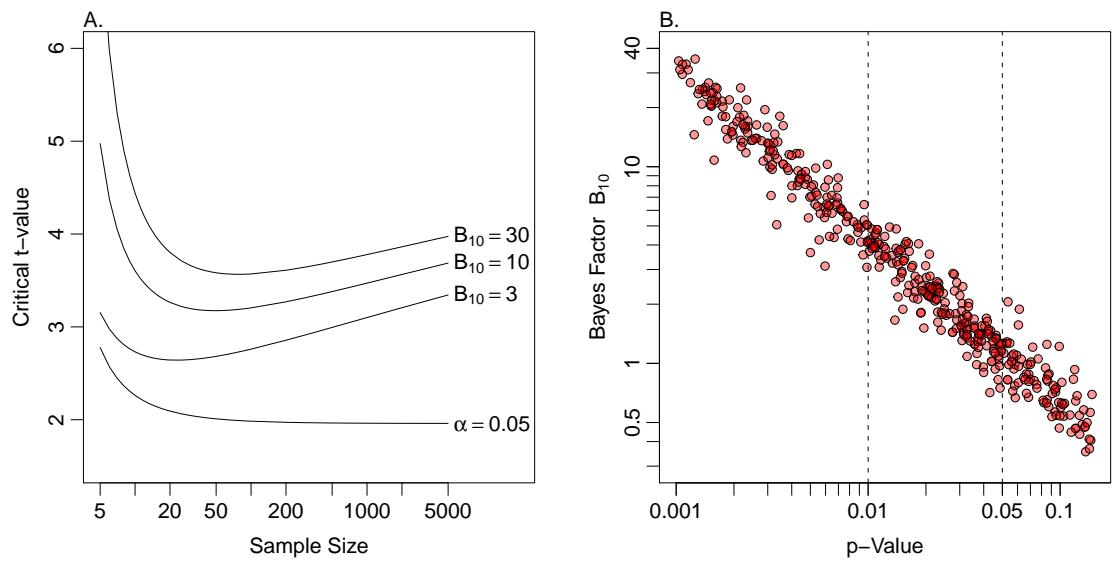
Figure 2: A. Needed t -values for stating evidence for an effect as a function of sample size. The lower line shows the needed t -values for p -value of .05. The upper lines are the t -values corresponding to B_{10} = 3, 10, 30 . B. Bayes factor evidence as a function of p -value for 855 t -tests reported in 2007 (adapted from Wetzels et al., 2011.)
