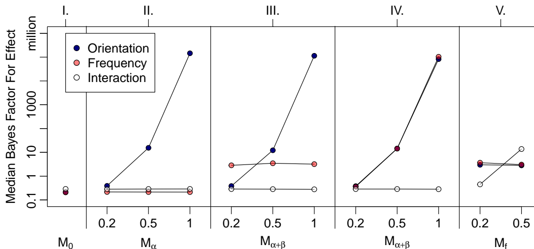
Figure 4: Median Bayes factor from simulated data. I. Data generated from the null model. II. Data generated with main effects in orientation. True effect-size values for orientation were .2, .5, and 1. III. Same as previous simulation, except there was a true main effect of frequency as well (true orientation effect-size values of .2, .5, and 1; true frequency effect-size value of .4). IV. Data generated with equal-sized true main effects in orientation and frequency. V. Data generated with main effects of both factors (true effect-size values of .4) and an interaction (true effect size values of .2 and .5). Orientation and frequency are modeled as fixed effects.
