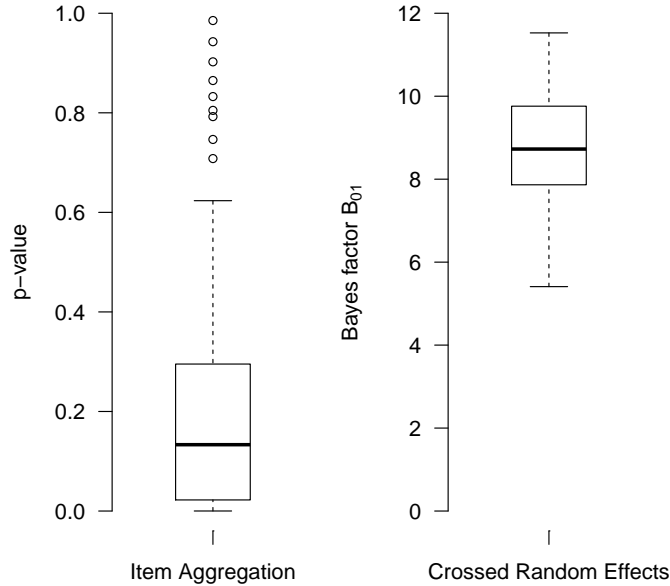
Figure 6: Simulation of a word-naming experiment with systematic variation across participants and items. Data were generated from a null model in which there was no part-of-speech effect. The p -values are obtained from a t -test on participant-specific noun and verb means. The distribution of these p -values deviates substantially from a uniform, with an overrepresentation of small values. The Bayes factors are from the same data, but the model includes crossed random effects of people and items. The Bayes factor favors the no part-of-speech effect null model.
