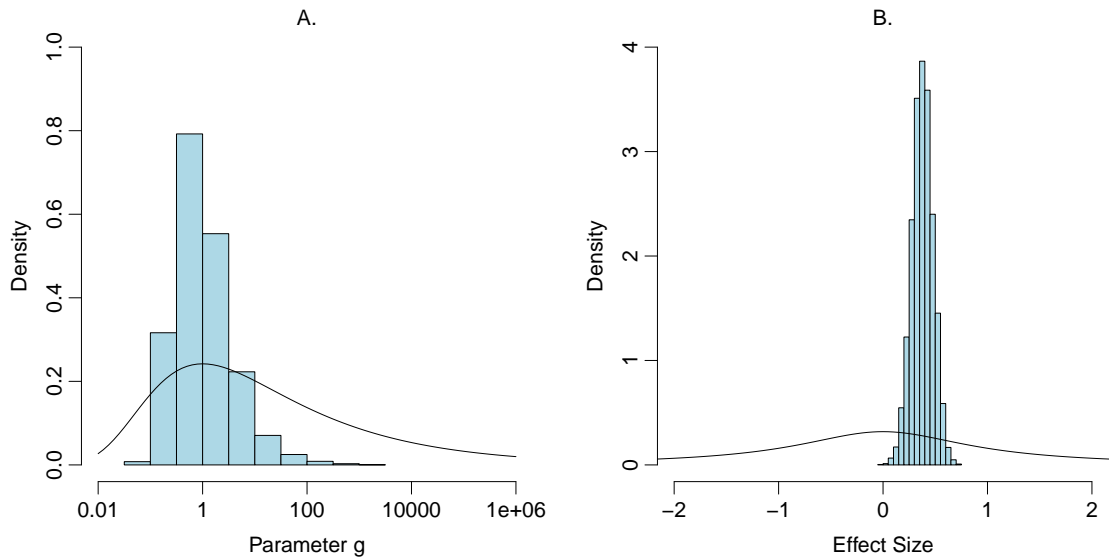
Figure 7: Concentration of posterior relative to the prior. A. The posterior for g is not too concentrated relative to its prior, and Monte Carlo integration is relatively efficient. B. The posterior for effect-size ( \alpha ) is more concentrated relative to prior, indicating that the closed-form integration over effects and variance is very helpful. The figure shows the case for a two-group design with 100 observations in each group. The model is a one-way, fixed effects model with four parameters: \mu , \sigma^2 , \alpha and g .
