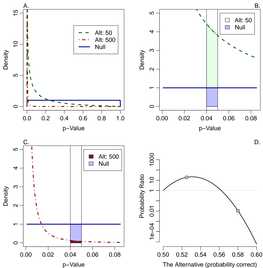
Figure 1: Significance tests overstate the evidence against the null hypothesis. A. The distribution of p -values for an alternative with effect-size of .2 (dashed and dashed-dotted lines are for sample sizes of 50 and 500, respectively) and the null (solid line). B. Probability of observing a p -value between .04 and .05 for the alternative (effect size = .2) and null for N = 50 . The probability favors the alternative by a ratio of about 4 to 1. C. Probability of observing a p -value between .04 and .05 for the alternative (effect size = .2) and null for N = 500 . The probability favors the null by a factor of 10. D. The probability ratio as a function of alternative. The probability ratio is the probability of observing a t -value of 2.51 and N = 100 given an alternative divided by the probability of observing this t -value for N = 100 given the null. The circle and square points highlight alternatives for which the ratios favor the alternative and null, respectively.
