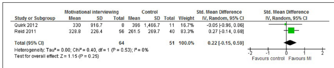
Figure 5. Forest plot of comparison physical activity cardiovascular conditions.
