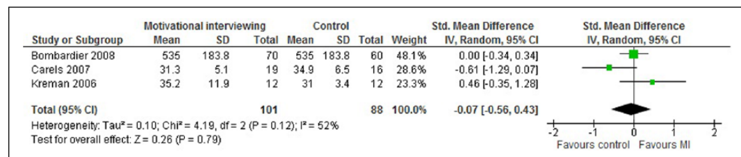
Figure 6. Forest plot of comparison cardiorespiratory fitness.
