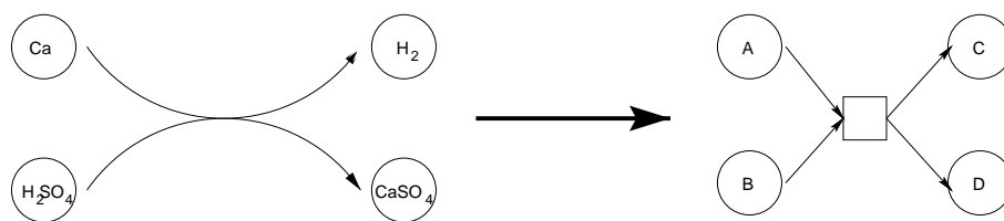
Figure 3: Encoding reaction (8) using a directed bipartite graph.
