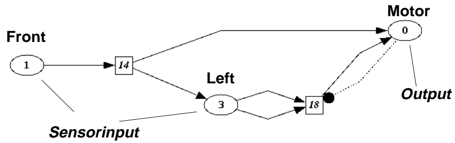
Figure 13: The kernel of the resulting artificial chemistry. The total graph has nearly 50 nodes and 70 edges and is not shown here. The kernel is labeled according to the function of the nodes. The dotted line indicates a catalytic effect.
