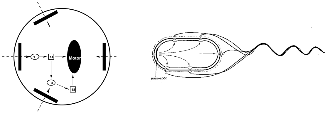
Figure 14: Left: The reaction network of the best individual as it is connected with the sensors and actuators of the robot. Note that the non-functional parts of the genome are omitted.
