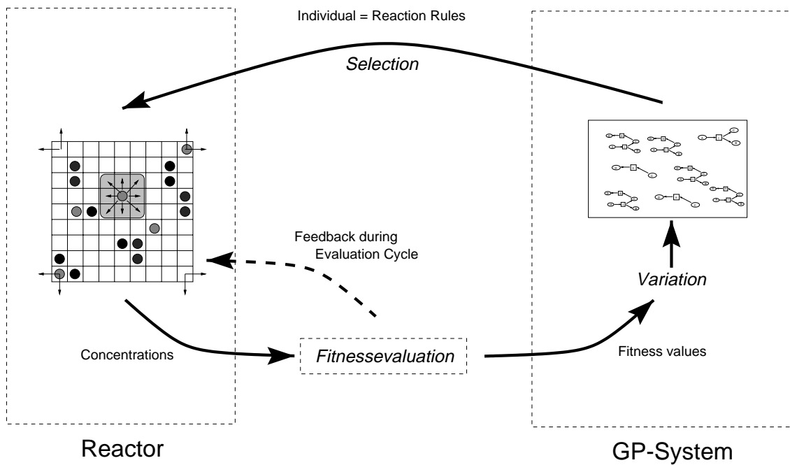
Figure 7: Schematic view of the evolutionary process.
