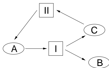
Figure 4: A chemically impossible reaction mechanism.
