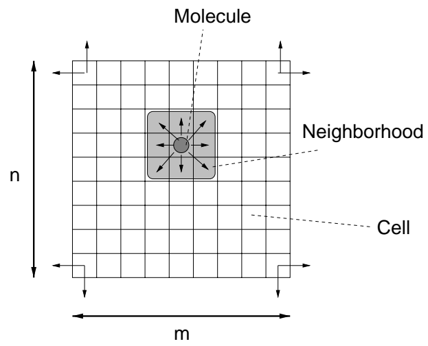
Figure 2: Neighborhood and diffusion of molecules.
