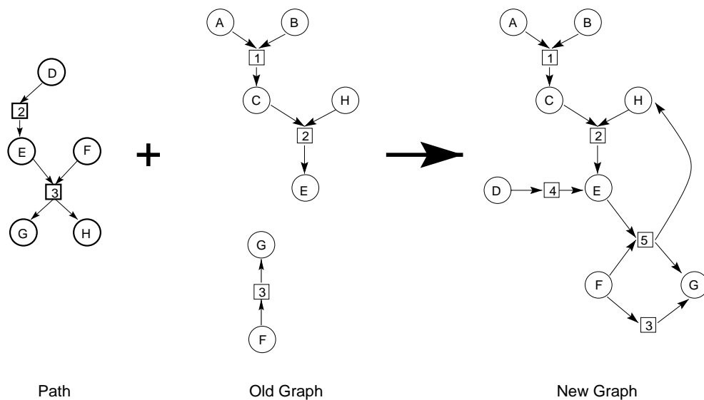
Figure 6: Inserting a pathway into a reaction graph. The reactions of the pathway are inserted into the graph. Missing nodes are created (e.g. node "D"). All existing reactions, molecules, and edges remain unchanged. Graph and pathway are shown without inhibitive/catalytic edges.
