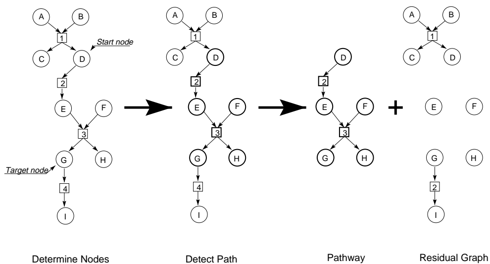
Figure 5: Detecting a pathway in a reaction graph. From left to right: (i) The start node and the target node are set. (ii) Depth-first search from start node to target node determines the path. (iii) The pathway is extracted from the reaction graph, including all necessary nodes. (iv) The pathway is deleted from the reaction graph. Graph and pathway are shown without inhibitive/catalytic edges.
