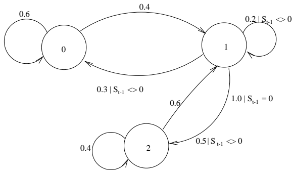
Figure A.5: Example 5. Higher order Markov chain before introducing higher order states.
