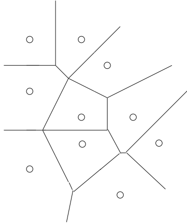
Figure 7.2: (A) A Voronoi tessellation of the input space derived from using WTA and the locations of a set of cells (shown as circles). In between each two cells, there is a hard decision boundary. The constructed tessellation determines those regions of the input space for which a particular cell is used (is activated) for returning its output.
