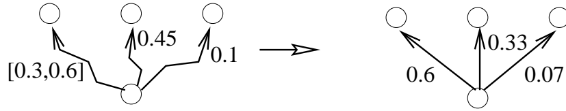
Figure 5.2: Model-Based Interval Estimation changes the transition probability of the best transition from a state/action pair to its upper probability bound. After this, the other transition probabilities are renormalized.
