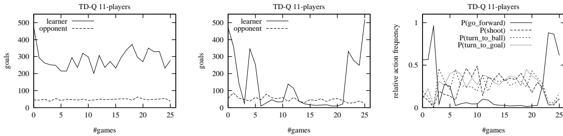
Figure 7.7: Performance breakdown study. Left: average numbers (means of 10 runs) of goals scored against BRO by a team with 11 players starting out with a well-trained linear network. Middle: plot for a single run. Right: relative frequencies of actions selected during the single run.
