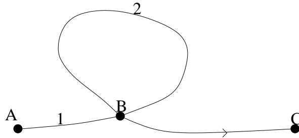
Figure 3.6: An example trajectory through state space. The Markov chain consists of three (abstracted) states A , B and C . At B , the chain can return to B or go to C .
