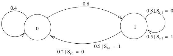
Figure A.3: Second order Markov chain before introducing higher order states.
