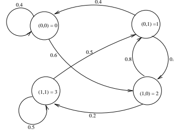
Figure A.4: The resulting Markov chain of figure 2 after converting the chain to higher order states and transitions.
